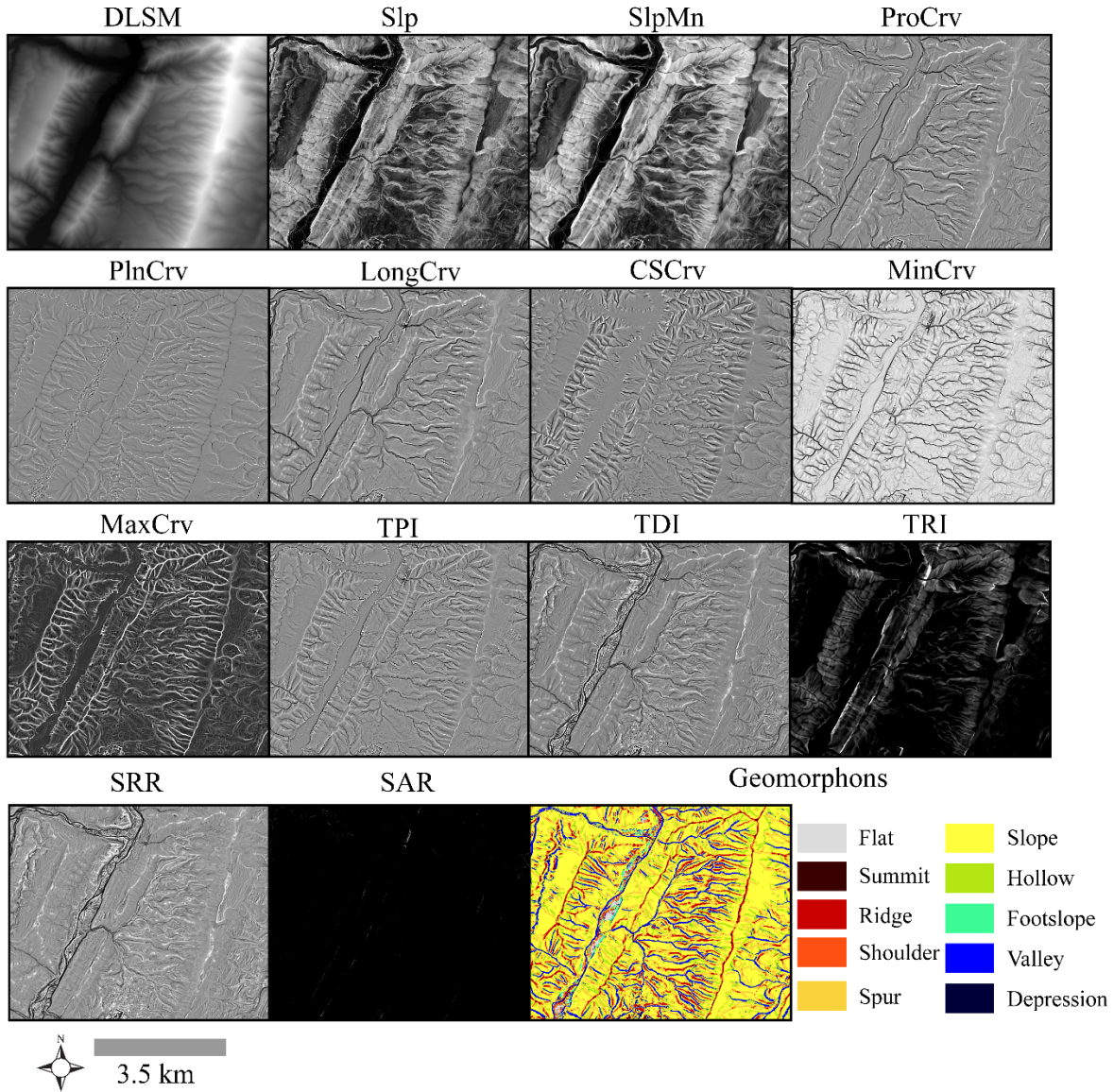
Figure 3. Example metrics that characterize local relief, terrain shape, and landforms. DLSM = digital land surface model, Slp = topographic slope, SlpMn = mean topographic slope, ProCrv = profile curvature, PlnCrv = plan curvature, LongCrv = longitudinal curvature, CSCrv = cross-sectional curvature, MinCrv = minimum curvature, MaxCrv = maximum curvature, TPI = topographic position index, TDI = topographic dissection index, TRI = topographic roughness index, SRR = surface relief ratio, and SAR = surface area ratio. Surface curvatures, TPI, and geomorphons were calculated using SAGA (Olaya and Conrad, 2009). Slp was calculated using ArcGIS Pro (“ArcGIS Pro help—ArcGIS Pro | Documentation”) while all other measures were calculated using R (R Core Team, 2020) and the spatialEco package (Evans, 2020).
