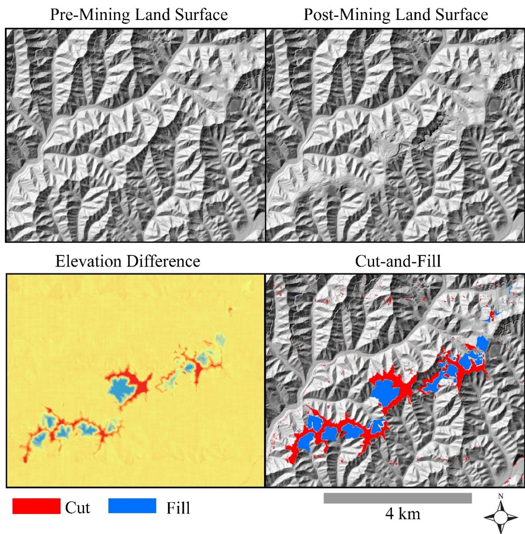
Figure 11. Example multi-temporal DLSM analysis to assess topographic change resulting from surface coal mining in southern West Virginia, USA. The pre- and post-mining land surfaces were derived from LiDAR point clouds provided by the West Virginia GIS Technical Center (WVGISTC).
