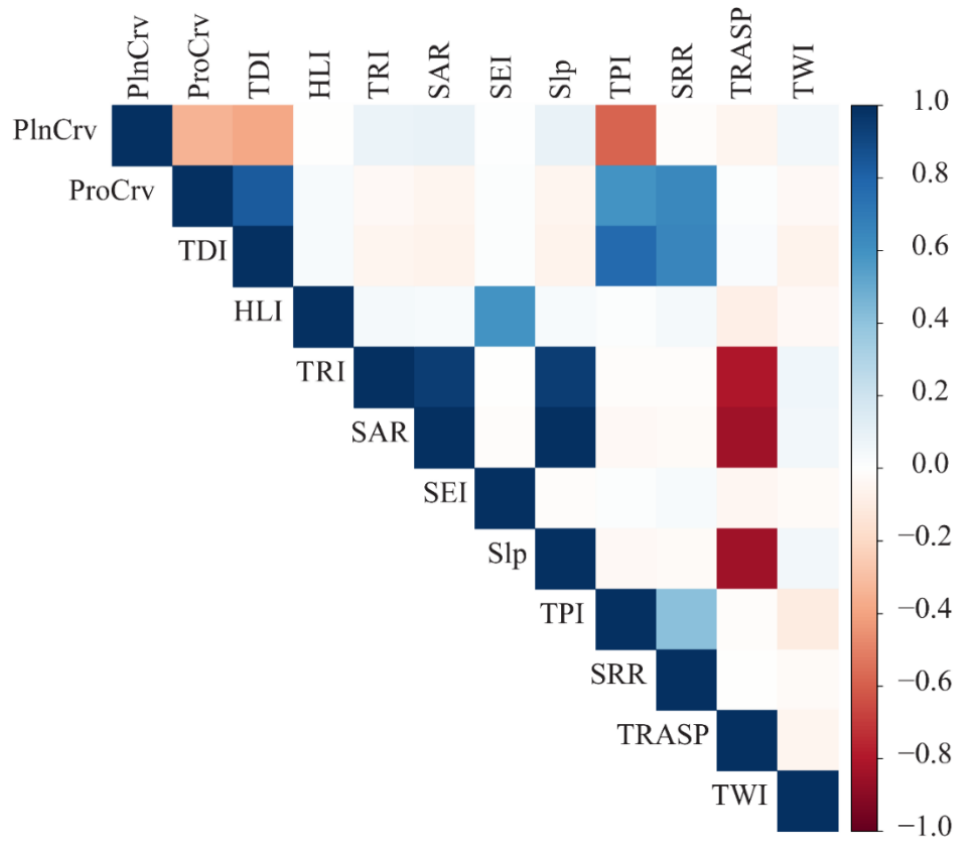
Figure 6. Correlation matrix for a set of 12 land-surface parameters derived from a DLSP. Darker red indicates a stronger negative correlation while darker blue indicates stronger positive correlation. Correlation was calculated using Spearman's rank correlation.
