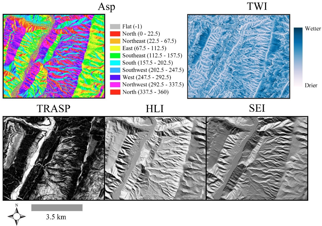
Figure 4. Example metrics that characterize solar insolation and moisture. Asp = slope aspect, TWI = topographic wetness index, TRASP = topographic radiation aspect index, HLI = head load index, and SEI = site exposure index. Asp was calculated using ArcGIS Pro (“ArcGIS Pro help—ArcGIS Pro | Documentation” ) while TRASP, HLI, and SEI were calculated using the spatialEco (Evans, 2020) package in R (R Core Team, 2020). TWI was calculated using SAGA (Olaya and Conrad, 2009).
