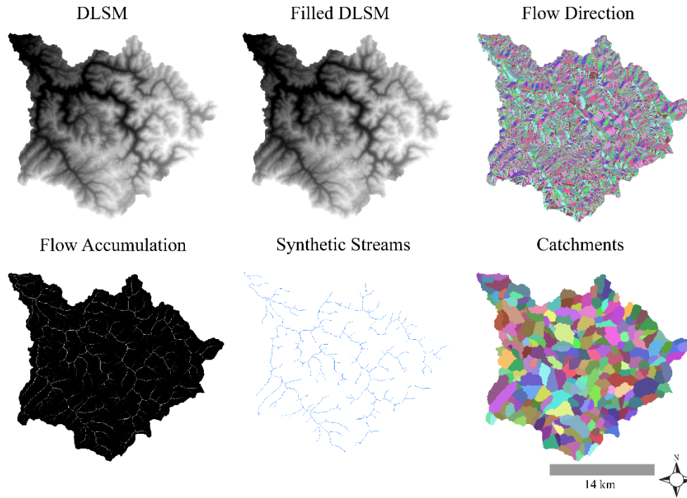
Figure 5. Example surface hydrologic derivatives. All metrics were calculating using ArcGIS Pro (“ArcGIS Pro help—ArcGIS Pro | Documentation” ). Results are for a catchment in West Virginia, USA.
