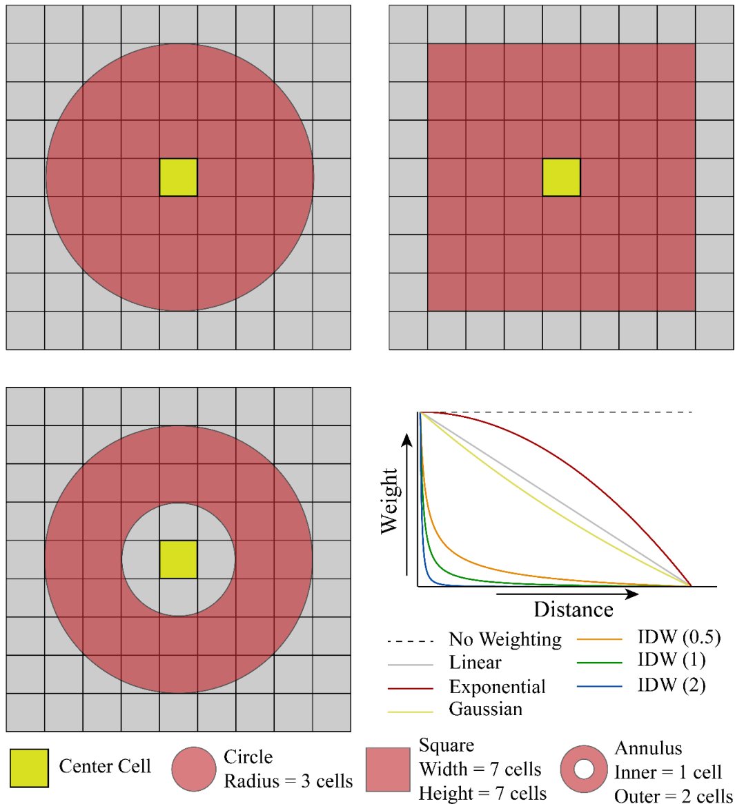
Figure 9. Example window shapes and distance weighting methods.
