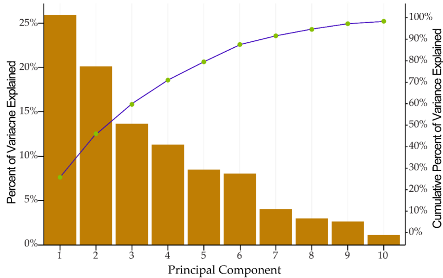
Figure 7. Scree plot describing the percent of variance in the original variables explained by the first ten principal components.
