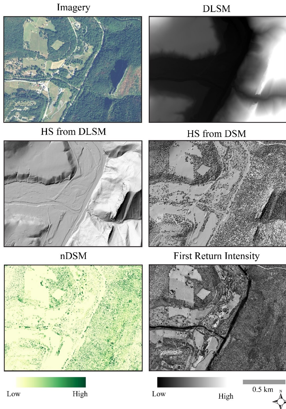
Figure 1. Example variables derived from LiDAR data. Image data are provided for comparison and are from the National Agriculture Imagery Program (NAIP). DLSM = Digital Land Surface Model, DSM = Digital Surface Model, nDSM = normalized Digital Surface Model. The DLSM and DSM are visualized using a hillshade (HS). All LiDAR derivatives were generated using ArcGIS Pro (“ArcGIS Pro help—ArcGIS Pro | Documentation”).
