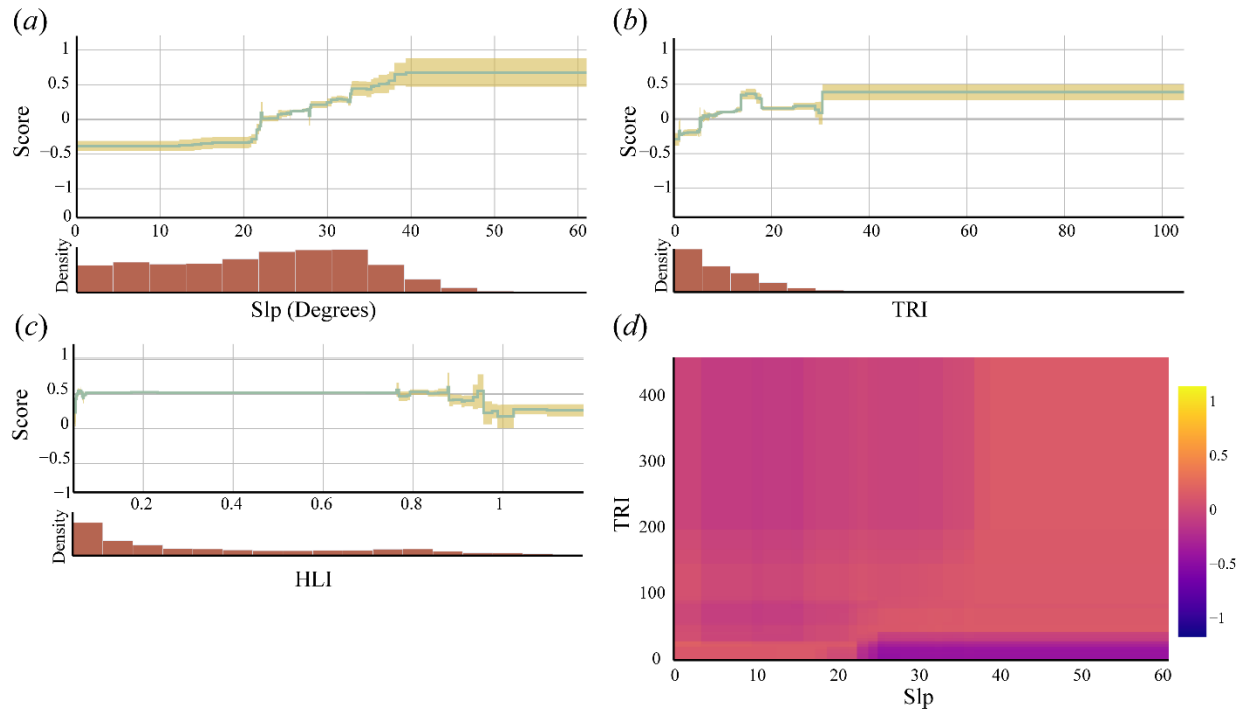
Figure 8. Example plots associated with explainable boosting machines (EBM). A score of 1 indicates a predicted high likelihood of slope failure occurrence while -1 indicates a high likelihood of not slope failure occurrence. (a) Slope (Slp) impact on resulting prediction. (b) Topographic roughness index (TRI) impact on resulting prediction. (c) Heat load index (HLI) impact on resulting prediction. (d) Interaction between Slp and TRI.
