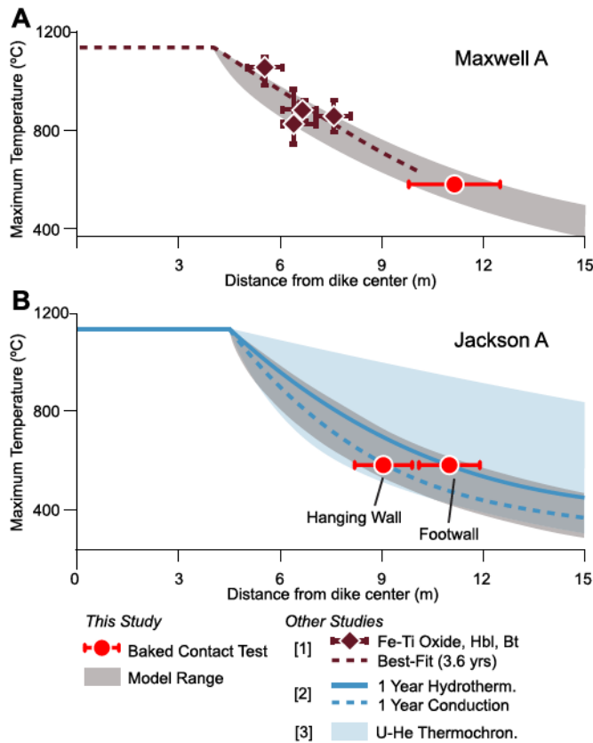
Fig. 7. A) MGT results from the Maxwell A dike (red circles) compared to Fe-Ti oxide, hornblende, and biotite results from [1] Petcovic and Gruner (2003). The range of model solutions from this study that are in agreement paleomagnetic results is shown in grey. B) MGT results from the Jackson A dike (red circles). Greater D_c in the footwall side of the dike might arise from the non-planar dike geometry seen in Fig. 2a, or reflect asymmetric heat transport efficacy below versus above the dipping dike structure. [2] Hydrothermal convection and conduction simulations from Bindeman et al. (2020) matching \delta^{18}\text{O} depletion profile around the dike. [3] (U-Th)/He thermochronology 68% confidence envelope of >10^6 simulations from Karlstrom et al. (2019).
