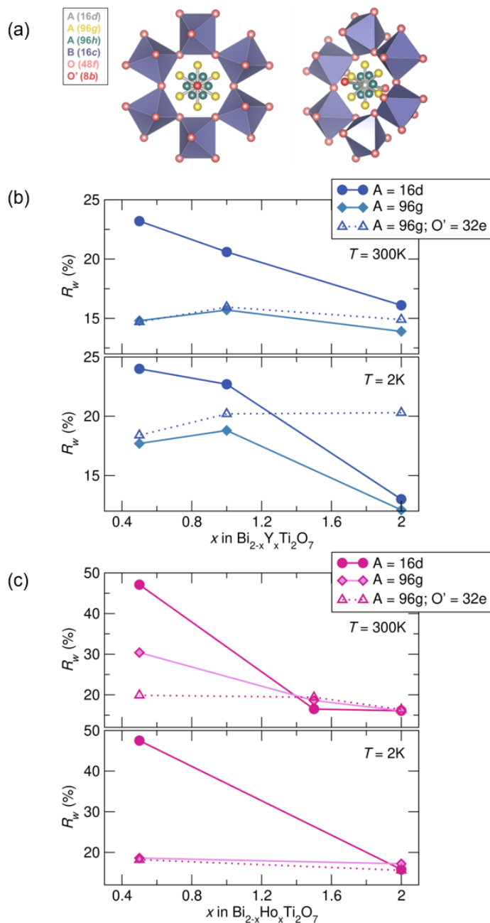
Fig. 3 (a) Various crystallographic sites in the split-site models for the A cation and O'. Note the 32e site is a variable site between the 8b (in red) and 16d (in grey) sites. R_w as a function of x in \text{Bi}_{2-x}\text{RE}_x\text{Ti}_2\text{O}_7 for (b) \text{RE}=\text{Y} and (c) \text{RE}=\text{Ho} (NPDF, NOMAD, SNS).
