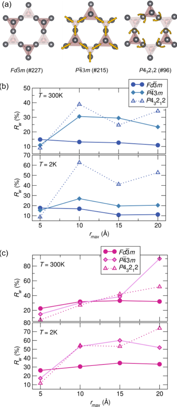
Fig. 5 (a) Distortions of the A-site cations in the various structural models. R_w as a function of box-car r_{max} for (b) \text{Bi}_{1.5}\text{Y}_{0.5}\text{Ti}_2\text{O}_7 at 300 and 2 K and (c) \text{Bi}_{1.5}\text{Ho}_{0.5}\text{Ti}_2\text{O}_7 at 300 and 2 K (NPDF, NOMAD, SNS).
