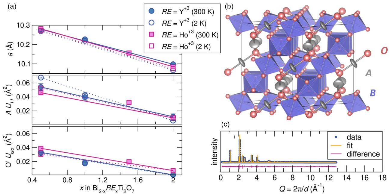
Fig. 1 (a) Summary of parameters from the Rietveld refinements (neutron, NOMAD, SNS; X-ray, 11BM, APS) against the cubic Fd\bar{3}m structure: lattice parameter (top), A -site U_{11} (middle), and O' site U_{iso} as a function of x in series \text{Bi}_{2-x}\text{RE}_x\text{Ti}_2\text{O}_7 . (b) Visualization of the cubic pyrochlore structure with refined atomic displacement parameters with ellipsoids shown at 90% probability. (c) Representative fit of the 11BM x-ray diffraction data for \text{Bi}_{1.5}\text{Y}_{0.5}\text{Ti}_2\text{O}_7 .
