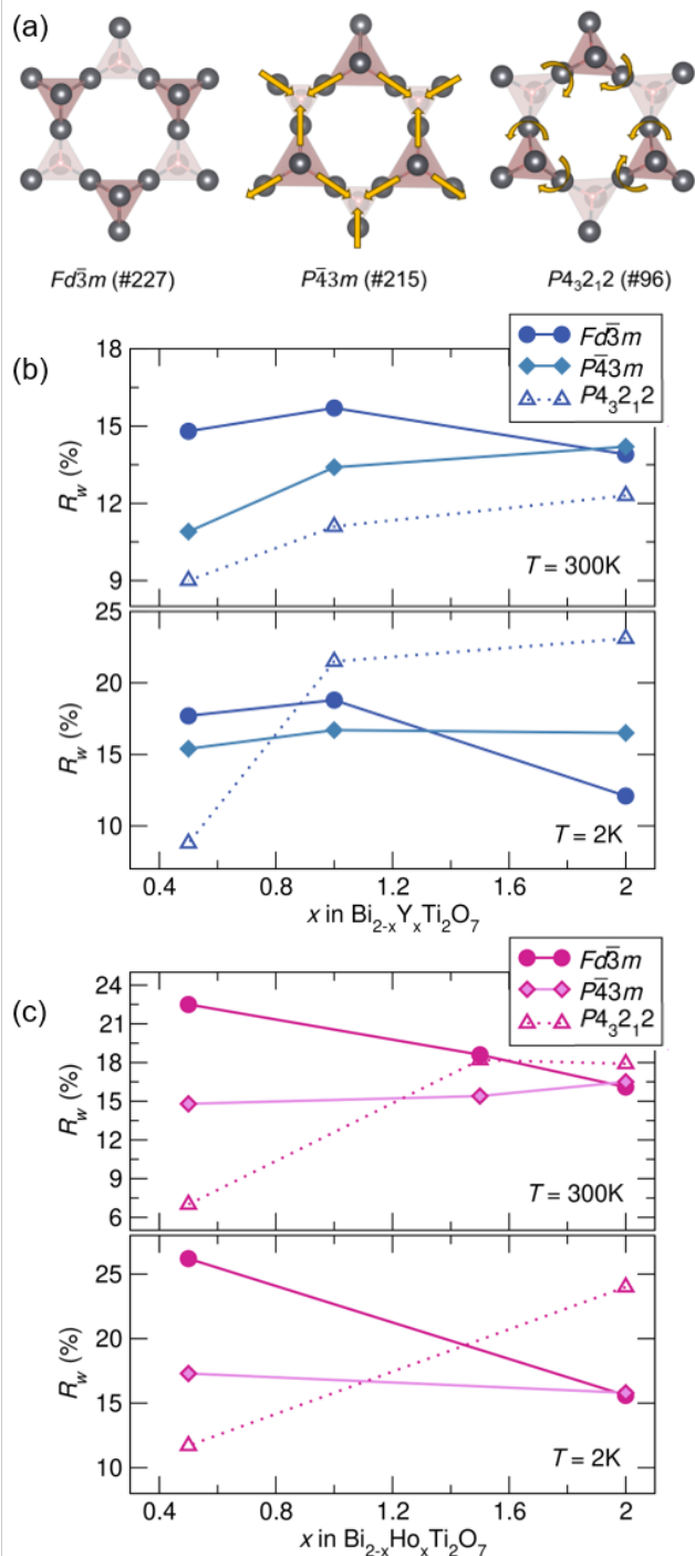
Fig. 4 (a) Distortions of the A-site cations in the various structural models. R_w as a function of x in \text{Bi}_{2-x}\text{RE}_x\text{Ti}_2\text{O}_7 for (b) \text{RE}=\text{Y} and (c) \text{RE}=\text{Ho} (NPDF, NOMAD, SNS).
