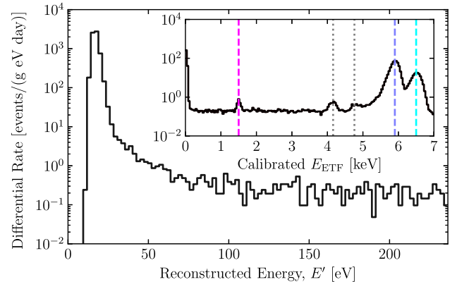
FIG. 2. Measured energy spectrum in the DM-search ROI for the full exposure after application of the quality cuts. The data have been normalized to events per gram per day per eV and have been corrected for the event-selection efficiency, but not the trigger efficiency. The inset shows the calibrated E_{\text{ETF}} spectrum up to 7 keV, noting the locations of the different spectral peaks. The known values of the dashed lines are 1.5, 5.9, and 6.5 keV for the Al fluorescence (pink), ^{55}\text{Fe} K_{\alpha} (blue), and ^{55}\text{Fe} K_{\beta} (cyan) lines, respectively. The two dotted gray lines between 4 and 5 keV in calibrated E_{\text{ETF}} are the Si escape peaks [29].
