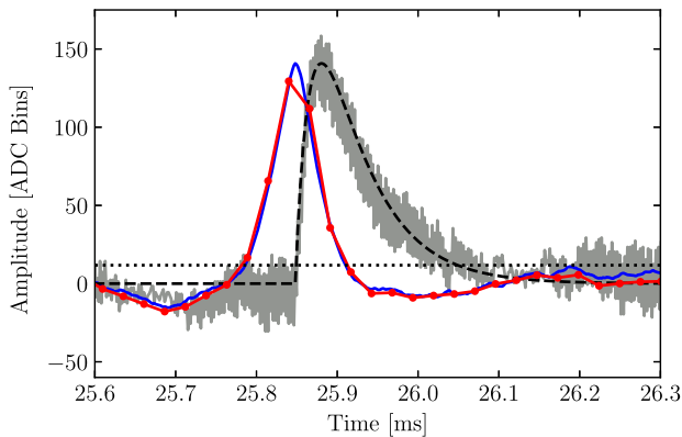
FIG. 1. A zoomed-in portion of an example event within the analysis ROI. The raw pulse (gray) is compared to the off-line optimal filter result (blue line), the pulse template scaled by the fit result (black dashed line), the FPGA filter result (red line with dots), and the FPGA trigger threshold (black dotted line). The off-line and FPGA optimal filters are highly correlated, but not exactly the same, with corresponding energy estimates for this event of 187 eV and 179 eV, respectively. The offset between the optimal filters and the raw pulse is an artifact of the filters, as they were set up to determine the time of the beginning of the pulse, as opposed to the maximum of the pulse.
