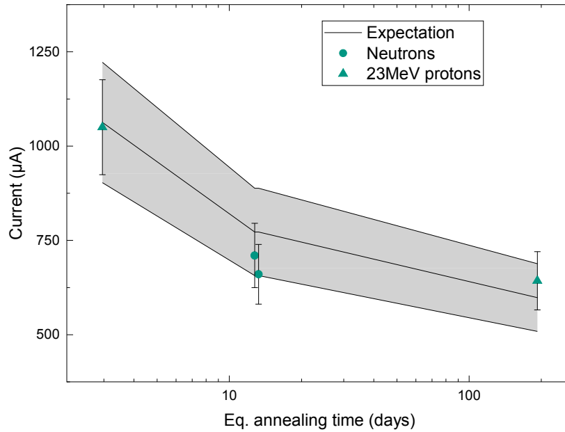
Figure 15. Currents measured at 20^\circ\text{C} and 600 V of the four irradiated full-size 2S sensors of type FZ290 over an estimated room temperature annealing time. The measurement of the temperature has an uncertainty of 0.5^\circ\text{C} , which propagates into the indicated uncertainty of the current at 20^\circ\text{C} . The expectation is calculated from the current-related damage rates given in ref. [26] with an uncertainty (indicated as grey band) on the fluence of 15%. The two circles representing the two sensors irradiated with neutrons have the same annealing time but are displaced in the plot for clarity.
