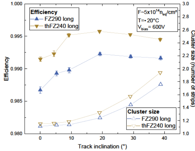
Figure 23. Efficiency (left axis) and cluster size (right axis) versus the inclination angle of the incident particles for the sensors on MiMo3 irradiated to a fluence of 5.0 \times 10^{14} n_{eq}/cm^2 and 203 days equivalent annealing at +21^\circ C . The module was operated at -20^\circ C and at a threshold of about 3450 e^- in the beam test.
