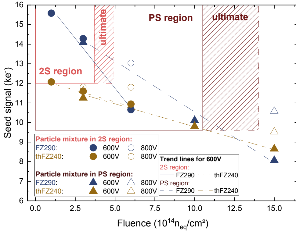
Figure 18. Seed signal of FZ290 (blue) and thFZ240 (brown) sensors for different fluences, measured at a temperature of 20^\circ\text{C} , interpolated to an equivalent annealing of 20 weeks at room temperature. Areas are indicated that represent the signal range required for strip sensors in the 2S and PS region. The solid markers represent measurements conducted at 600 V. Measurement results conducted at 800 V are added in case the initially measured signal is below its specification in order to show the impact of increased bias voltage. The trend of the signals at 600 V for both materials are indicated by the lines.
