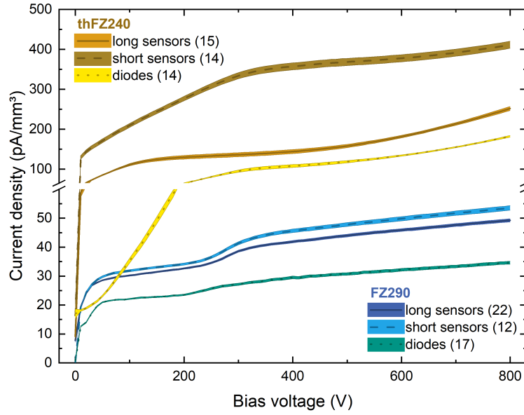
Figure 9. Averaged IV curves for mini-sensors and diodes prior to irradiation measured at 20 °C. The currents are normalized to the active volume of the devices. The numbers in the legend refer to the number of samples used to generate the averaged curve. For each bias voltage and sensor type the mean and standard deviation of the measured current was computed. The mean is plotted as the line and the bands represent one standard deviation.
