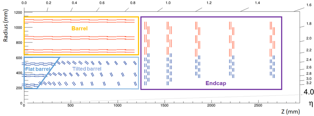
Figure 2. Cross-sectional view obtained by making a slice through one quadrant of the Phase-2 Outer Tracker at CMS in the R-Z plane. The beam line is along the Z -axis. The red lines represent 2S modules at larger radii and the blue lines the PS modules in the inner layers. These module types are described in the text below.
