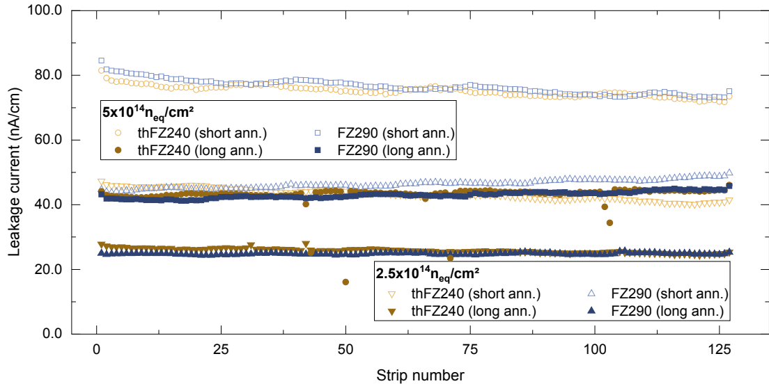
Figure 12. Leakage current vs. strip number measured at 20^\circ\text{C} and 350 V. The terms “short ann.” (equivalent to 9 days at 21^\circ\text{C} ; open symbols) and “long ann.” (equivalent to 200 days at 21^\circ\text{C} ; bold symbols) refer to the annealing time prior to the measurements. The data after a fluence of 2.5 \cdot 10^{14} \text{ n}_{\text{eq}} \text{ cm}^2 are represented by triangles and the data after 5 \cdot 10^{14} \text{ n}_{\text{eq}} \text{ cm}^2 with squares and circles.
