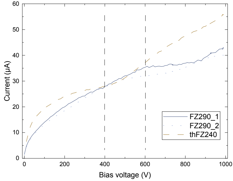
Figure 11. Comparison of the current vs. voltage characteristics for one thin (thFZ240) and two thick (FZ290) sensors irradiated to 1 \cdot 10^{15} \text{ n}_{\text{eq}} \text{ cm}^2 . The measurements were performed at 20^\circ\text{C} . The vertical lines indicate the bias voltages discussed in the text.
