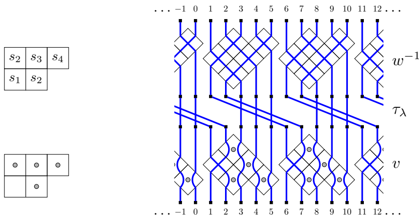
FIGURE 2. A J -diagram (bottom left), the labeling of its squares by simple transpositions (top left), and the result of applying the bijection of Theorem 9.3 (right). See Example 9.6 for details.
