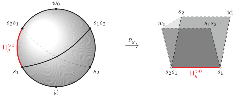
FIGURE 1. The map \bar{\nu}_g for the case G = \mathrm{SL}_3 and P = B from Example 1.4
