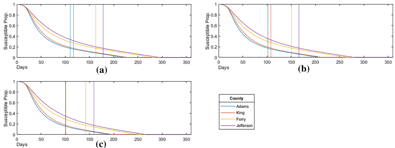
Figure 18. Susceptible proportion for: (a) the homogeneous priority distribution ( \omega = \omega_C ); (b) the moderate priority distribution ( \omega = \omega_M ); (c) the strict priority distribution ( \omega = \omega_S ).
