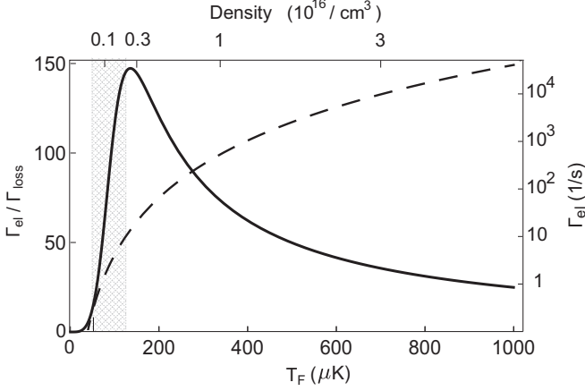
FIG. 1. The ratio of good (elastic) to bad (inelastic) collisions, and the elastic collision rate for ^6\text{Li} atoms near zero field, far away from the p -wave Feshbach resonance. The solid line shows the ratio for an harmonically trapped cloud with T = T_F assuming a vacuum lifetime of 60 seconds. The dashed line is the elastic collision rate. In this work, we have explored the shaded region.
