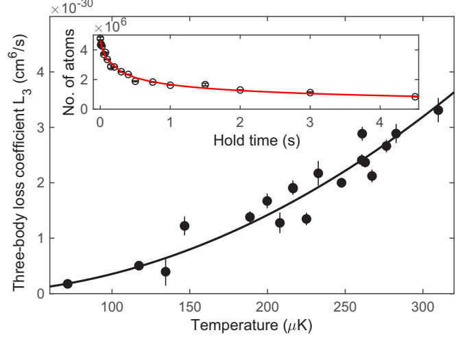
FIG. 2. Three-body loss for spin-polarized fermions. Different temperatures are realized by reducing the trap laser power. The three-body loss coefficient L_3 scales quadratically with temperature. The black line is a parabolic fit through the origin, resulting in L_3 = (3.55 \pm 0.22) \times 10^{-23} \times T^2 . Error bars show the statistical one standard deviation uncertainties of the fit parameter L_3 used to describe the atom number decay. The inset shows the decay curve at T = 310 \mu\text{K} and its fit to Eq. (1).
