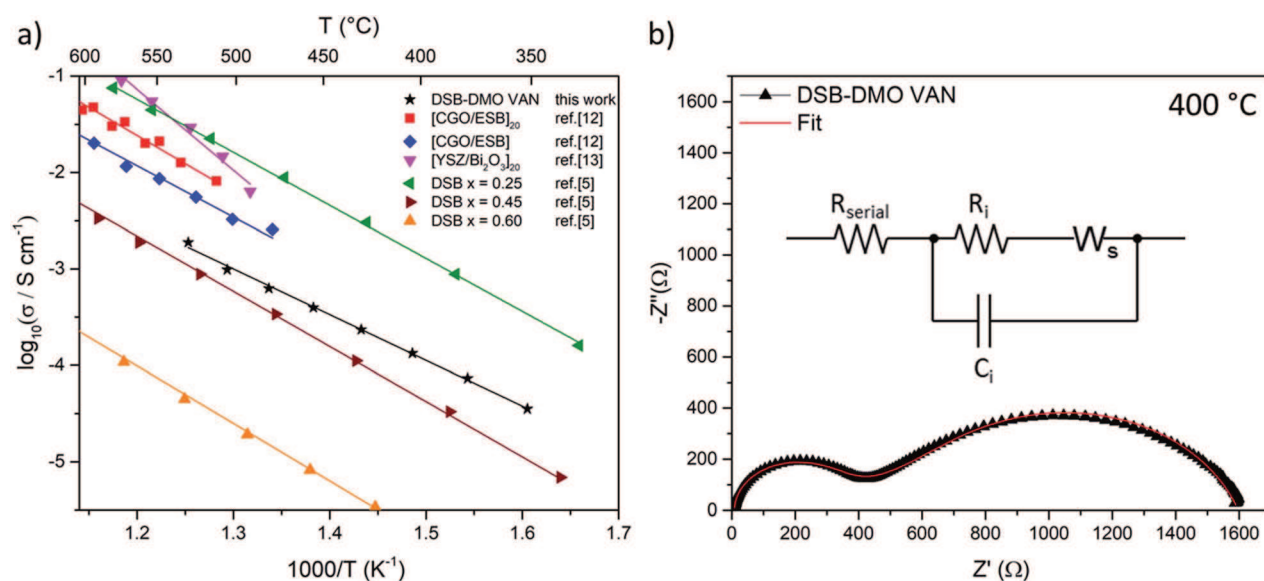
Fig. 3 (a) Arrhenius plot of DSB-DMO VAN film in air displaying high ionic conductivity as compared to the literature results for superlattices 12,13 and bulk powder DSB 5 (b) typical Nyquist plot at 400 °C. Inset: the Randles model used to fit the data, where R_i/C_i models the ionic conductivity of DSB, W_s the FLW response, and R_{\text{serial}} the internal resistances of the EIS setup.
