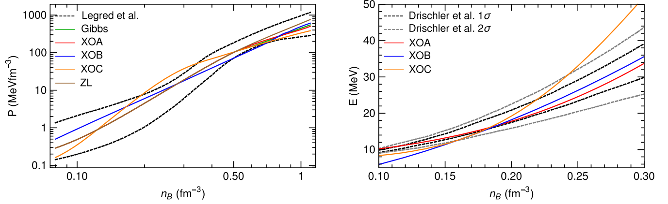
FIG. 2. Left panel: pressure versus baryon density as obtained by the assorted EOSs used herein compared with the astrophysical constraints of Legred et al. [34] (in black, dashed lines). All parametrizations meet these constraints successfully with the exception of XOC which fails to stay in the allowed region around 2.0n_{\text{sat}} , where n_{\text{sat}} = 0.16 \text{ fm}^{-3} . Right panel: energy per particle versus baryon density of beta-equilibrium matter for the various EOSs used in this work compared with the 1\text{-}\sigma and 2\text{-}\sigma constraints from Drischler et al. [23] obtained in a chiral EFT framework. Results corresponding to Gibbs and ZL are not shown because, over the range of densities displayed, they are identical to XOA. Only XOA remains within the 2\text{-}\sigma constraints of [23] up to \sim 2.0n_{\text{sat}} .
