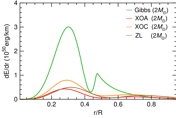
FIG. 11. Energy/unit distance of the fundamental g mode as a function of distance from the center for the ZL, XOA, XOC, and Gibbs EOS for a \sim 2 M_\odot star. Note that the mode energies in the ZL and crossover cases are scaled up by a factor of 10 for the purpose of comparison.
