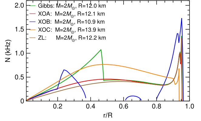
FIG. 8. The Brunt-Väisälä frequency in a hybrid star of mass 2.0 M_\odot for the Gibbs and crossover models. The Brunt-Väisälä frequency for the “good” crossover model XOA is very similar to the nucleonic ZL EOS (which includes muons), whereas the Gibbs model shows a distinct peak corresponding to the rapid onset of quark matter. Parameters for the nuclear and quark EOSs are as in Table I.
