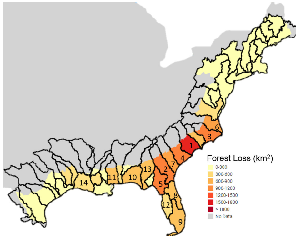
Figure 2. The area of coastal forested wetlands deforested within every hydrologic subregion (4-digit HUC codes) across the North American Coastal Plain is shown above. Subregions with forested coastal wetland area greater than 5000 km 2 in 1996 were ranked based on cumulative loss from 1996 to 2016, which is indicated by the number within a subregion (on the map and Table 1). Observed losses are concentrated in the Southeastern US (Louisiana to North Carolina). Subregions West of Louisiana and North of the Delmarva Peninsula had relatively few losses.
