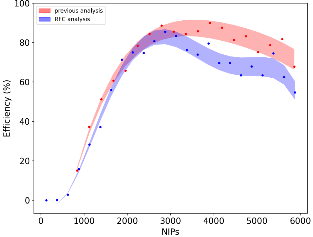
Figure 7. The detector efficiency as a function of NIPs for the previous and RFC analyses.
