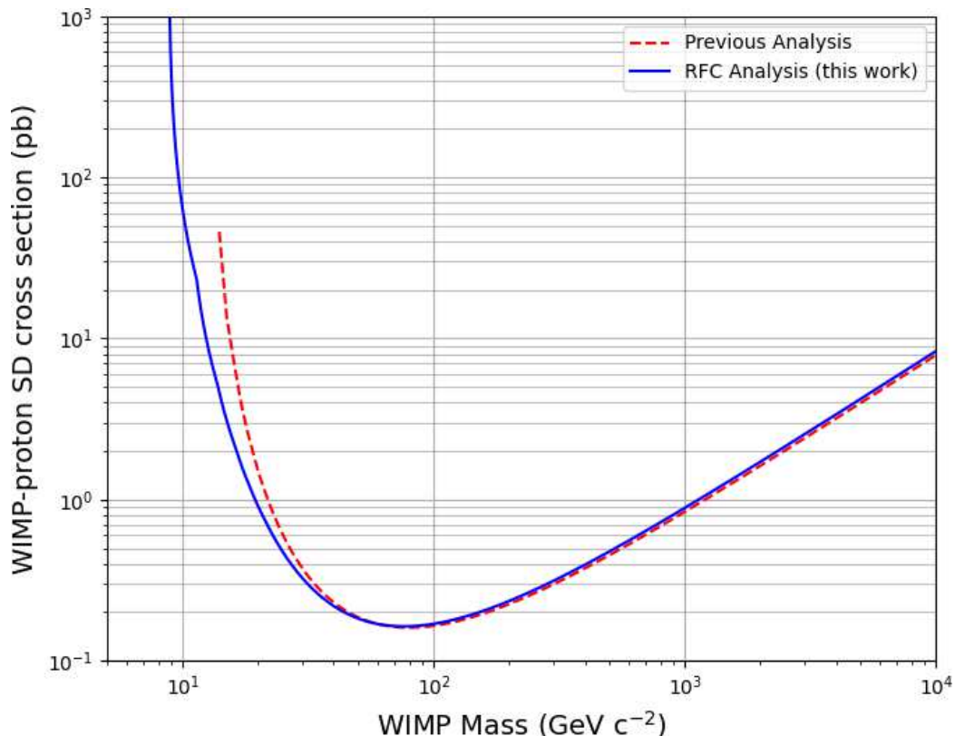
Figure 9. Projected DRIFT-IIcd SD WIMP exclusion limits for the previous [5] and RFC analyses, calculated for a hypothetical 100 day exposure using the analysis efficiencies from figure 7 and the methods and parameters described by ref. [21] and ref. [22].
