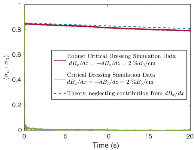
FIG. 9. Simulated signal for highly tuned RCD modulated at 200 \text{ Hz} (red) and CSD (green), with theoretical estimation for RCD (blue). The starting phase for ^3\text{He} is \phi_3 = \pi/8 , and it is the same for neutrons, \phi_n = \pi/8 . Signal is observable for a long time in the RCD scenario, while the signal is indistinguishable from noise in a traditional critical dressing scenario.
