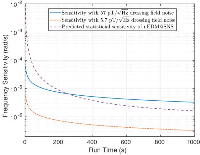
FIG. 1. Run-to-run uncertainty in the measured frequency due to dressing field noise for 57 and 5.7 pT/√Hz dressing field noise and a perfect band-pass filter around the dressing frequency, calculated from Eq. (76). The predicted per-run sensitivity for the nEDM@SNS, formulated from Ref. [9], is shown for comparison. It is shown that 57 pT/√Hz dressing field noise will significantly reduce the ultimate sensitivity of the measured frequency, while 5.7 pT/√Hz dressing field noise is acceptable.
