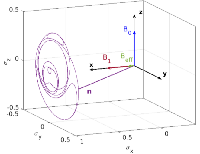
FIG. 6. A classical visualization of the neutron spin trajectory undergoing robust dressing on the Bloch sphere in the laboratory frame, with arrows representing the static uniform field B_0 , the dressing field B_1 , and the robust dressing effective field B_{\text{eff}} .
