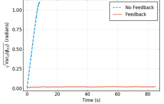
FIG. 4. The root-mean-square deviation of the angle between the neutron and ^3\text{He} spins ( \phi_{n3} ) as a function of time, with dressing field powered by a Kepco four-quadrant 400 36-12 power supply, for magnetic fields generated with (solid line) and without (dashed line) feedback control. The dataset without feedback consists of 28 runs, while the dataset with feedback consists of 50. Data are smoothed for clarity.
