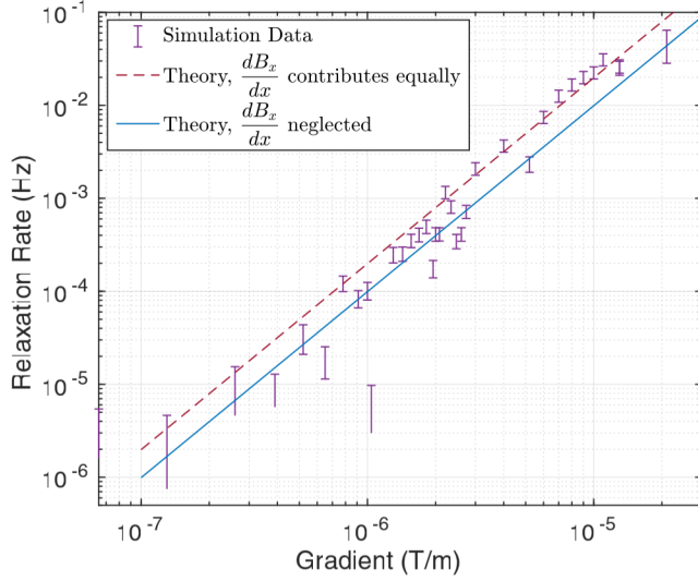
FIG. 7. Relaxation after optimization of robust dressing parameters for 200 Hz robust dressing and a wide range of gradient magnitudes. The gradients in this simulation arise from the divergence theorem, \frac{dB_z}{dz} = -\frac{dB_x}{dx} .
