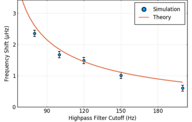
FIG. 3. Predicted and simulated frequency shifts, with magnetic field noise given by Eq. (83), for various high-pass filter cutoffs. The theory line is calculated from Eqs. (71) and (83). Each simulated point represents 100 000 neutrons.
