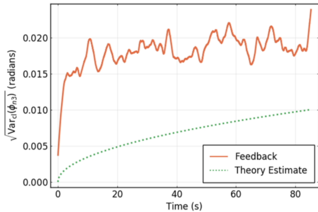
FIG. 5. Phase standard deviation with feedback control applied from the field powered by a Kepco four-quadrant 400 36-12 power supply (solid line). The rms phase deviation rises for a period of less than five seconds, then appears to settle near a fixed value. For comparison, the theoretical estimate (dotted line) is computed assuming 400 \text{ pT}/\sqrt{\text{Hz}} noise that is high-pass filtered at 500 Hz. Data are smoothed for clarity.
