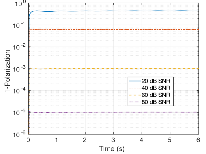
FIG. 8. 1-Polarization for robust dressing modulated according to Eq. (86), where B_1 = 40.2497 \mu\text{T} and \omega_m = 200 Hz, with simulated noise power varied from 20 to 80 dB SNR.
