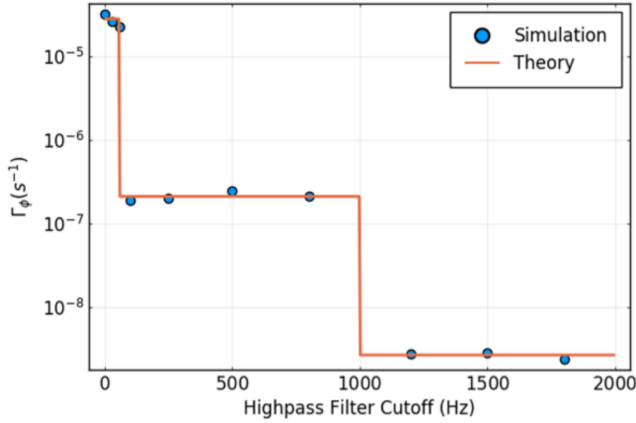
FIG. 2. Predicted and simulated values of \Gamma_\phi for various high-pass filter cutoffs. The theory line is calculated from Eqs. (70) and (83). Each simulated point represents 200 neutrons. Note that cutoff values beyond the dressing frequency (1000 Hz) are only achievable in simulation, and are shown here for comparison to the theory.
