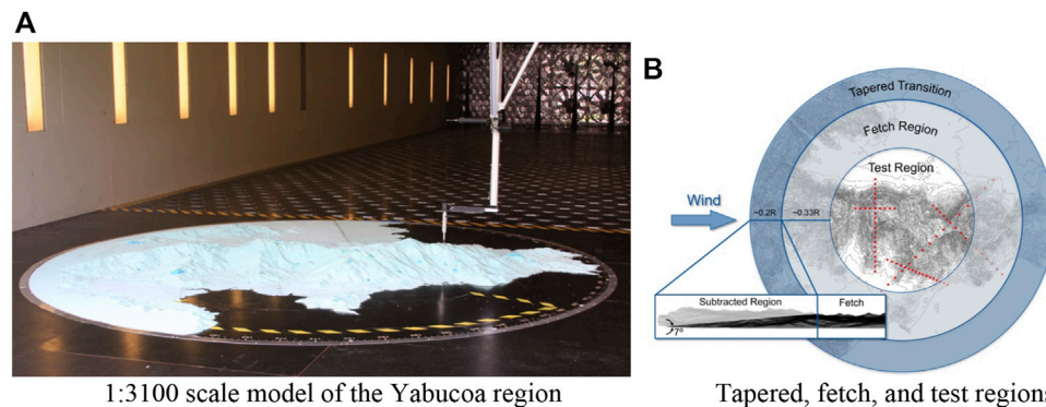
FIGURE 7 | Tapered, fetch, test regions and measurement locations of the model. (A) 1:3,100 scale model of the Yabucoa region. (B) Tapered, fetch, and test regions.
