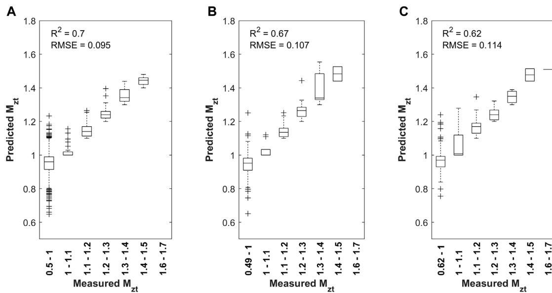
FIGURE 11 | Training, testing, and validation of a single layer, 30 neuron model for the smooth-to-rough transition cases using 100 m horizontal spacing DEM data. (A) Training, (B) Testing, and (C) Validation.
