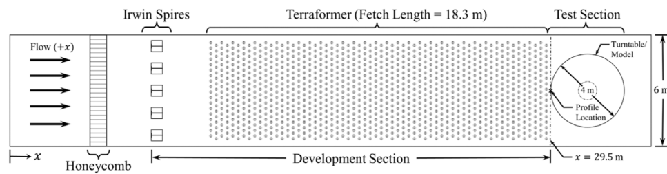
FIGURE 3 | Boundary Layer Wind Tunnel Configuration.
