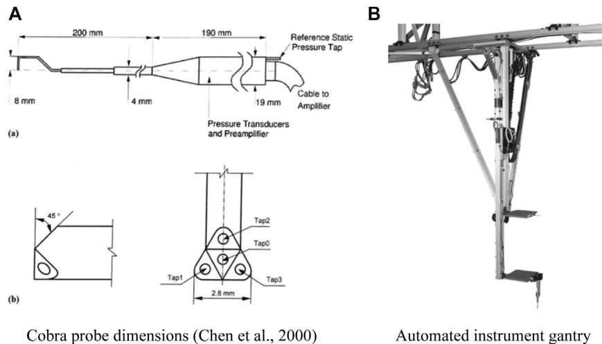
FIGURE 4 | Cobra probe instrumentation. (A) Cobra probe dimensions (Chen et al., 2000). (B) Automated instrument gantry.
