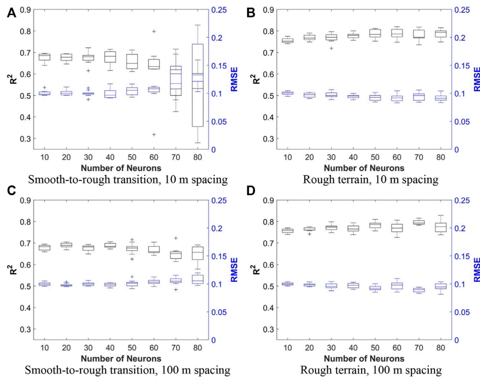
FIGURE 10 | Coefficients of determination for varied neuron counts and horizontal spacing between elevation data points in the DEM for the double layer neural network. (A) Smooth-to-rough transition, 10 m spacing. (B) Rough terrain, 10 m spacing. (C) Smooth-to-rough transition, 100 m spacing. (D) Rough terrain, 100 m spacing.
