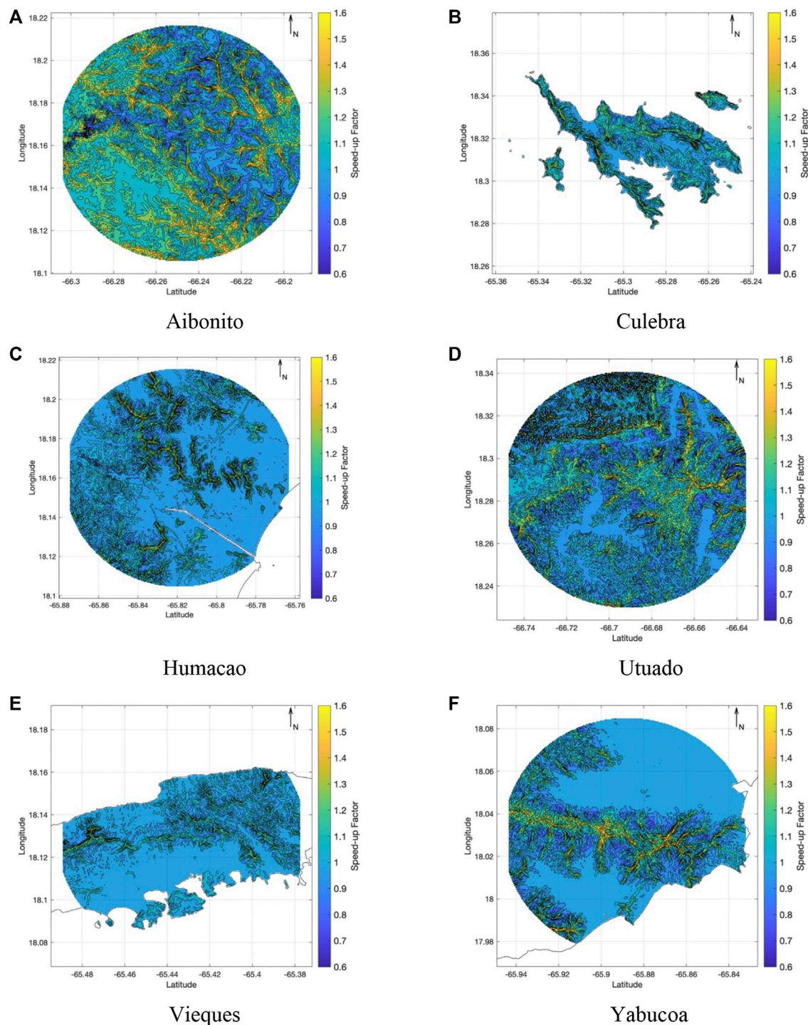
FIGURE 15 | Predictions of topographic effect multipliers, enveloping for all directions. (A) Aibonito. (B) Culebra. (C) Humacao. (D) Utuado. (E) Vieques. (F) Yabucoa.
