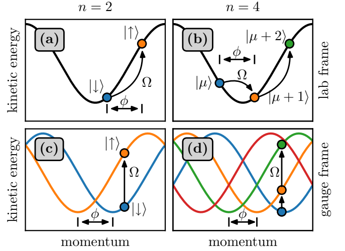
FIG. 4. Spin-orbit coupling for (a),(c) two-level and (b),(d) four-level spins. Colors indicate different spin projections \mu . (a),(b) In the “lab frame” kinetic energy is insensitive to spin, but a spin transition \mu \rightarrow \mu + 1 is accompanied by a momentum kick q \rightarrow q + \phi from the drive. (c),(d) Changing into the “gauge frame”, essentially by shifting the momentum label q for each spin state \mu , makes the drive diagonal in the momentum index, but comes at the cost of making kinetic energy spin-dependent.
