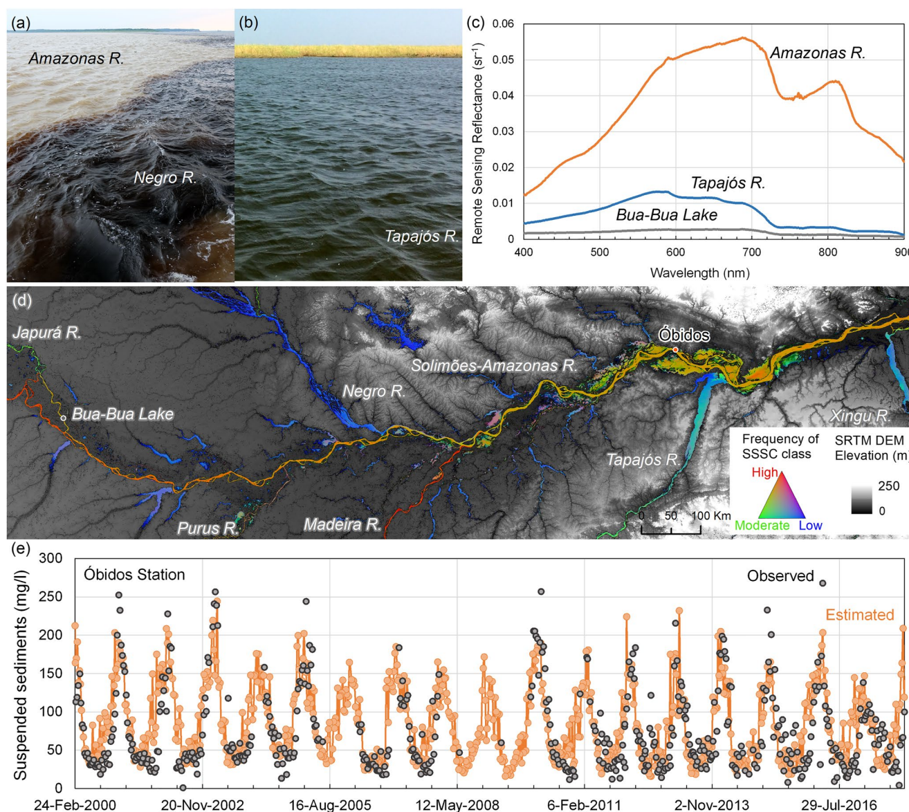
Figure 8. (a) Examples of white and black, and (b) Clear waters. (c) Examples of spectra of three water types (Source: Labisa; http://www.dpi.inpe.br/labisa/ ): white water - Amazon River (TSS of 288.5 \text{ mg L}^{-1} ; \text{Chl-}a of 2.0 \mu\text{g L}^{-1} ; a\text{CDOM} in 440 \text{ nm} of 1.3 \text{ m}^{-1} ); clear water—Tapajós River (TSS 5.7 \text{ mg L}^{-1} ; \text{Chl-}a of 10.8 \mu\text{g L}^{-1} ; a\text{CDOM} in 440 \text{ nm} of 1.2 \text{ m}^{-1} ); black water - Bua-Bua Lake (TSS 7.4 \text{ mg L}^{-1} ; \text{Chl-}a of 3.6 \mu\text{g L}^{-1} ; a\text{CDOM} in 440 \text{ nm} of 2.9 \text{ m}^{-1} ). (d) Spatial variability of suspended sediments in the central Amazon (adapted from Fassoni-Andrade & Paiva, 2019). (e) Suspended sediment time-series in situ (observed) and satellite-based Moderate Resolution Imaging Spectroradiometer (estimated) obtained from the HYBAM monitoring system ( http://hidrosat.ana.gov.br ).
