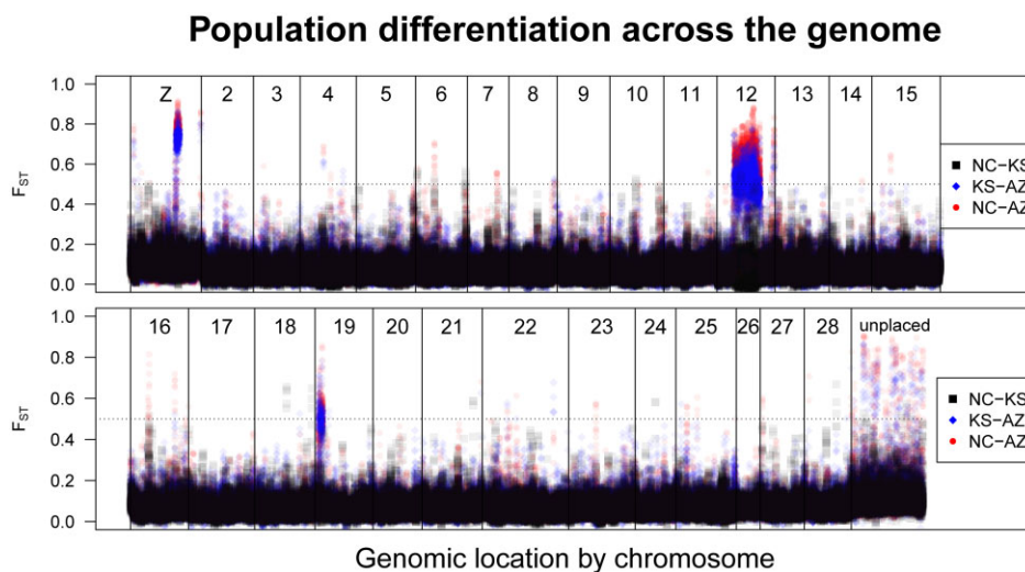
Fig. 3. Pairwise differentiation ( F_{ST} ) across the M. sexta genome: North Carolina (NC) versus Kansas (KS; black squares), Kansas versus Arizona (AZ; blue diamonds), and North Carolina versus Arizona (red points). Plotting is ordered by chromosomal linkage. For ease of visualization, the genome is split into 2 rows. We examined regions enriched for differentiation greater than 0.5 (dashed line). By this metric, one peak on the Z, and one peak each on chromosomes 12 and 19. Additionally, note that the highest peaks almost always come from KS versus AZ and NC versus AZ, indicating that Arizona's population is more distinct from the others than NC and KS are from each other. Chromosomes are numbered based on syntenic assignment of HiC scaffolds from the Gershman assembly. Unplaced scaffolds are all those beyond the 28 main chromosomal scaffolds.
