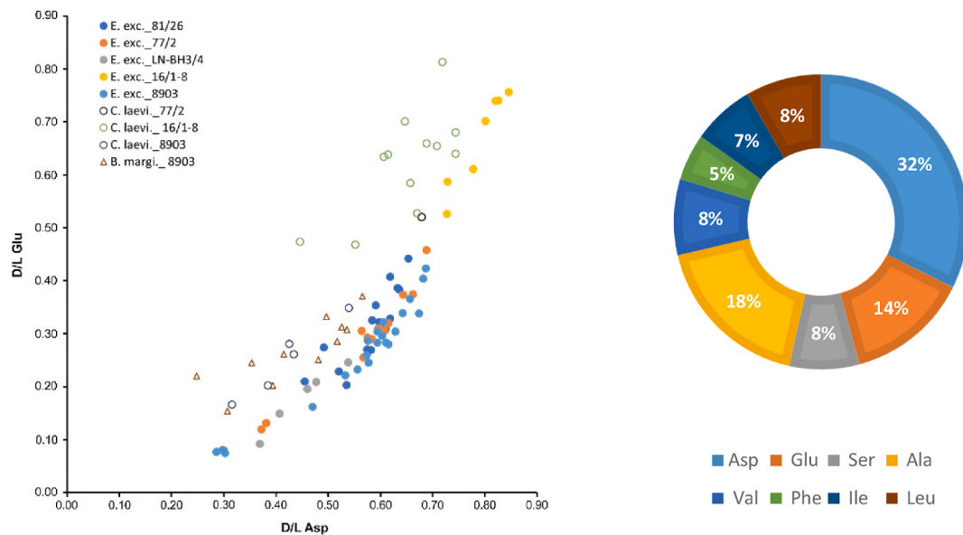
Fig. 4. a) Co-variance between D/L Asp and D/L Glu in three species ( Elphidium excavatum , Cassidulina laevigata and Buliminia marginata ) measured in four shallow borings (81/26; 77/2; LN-BH3/4 and 8903) and one well (16/1–8) b) Relative concentration of eight amino acids measured in individual subsamples of benthic foraminifera Elphidium excavatum before screening.
