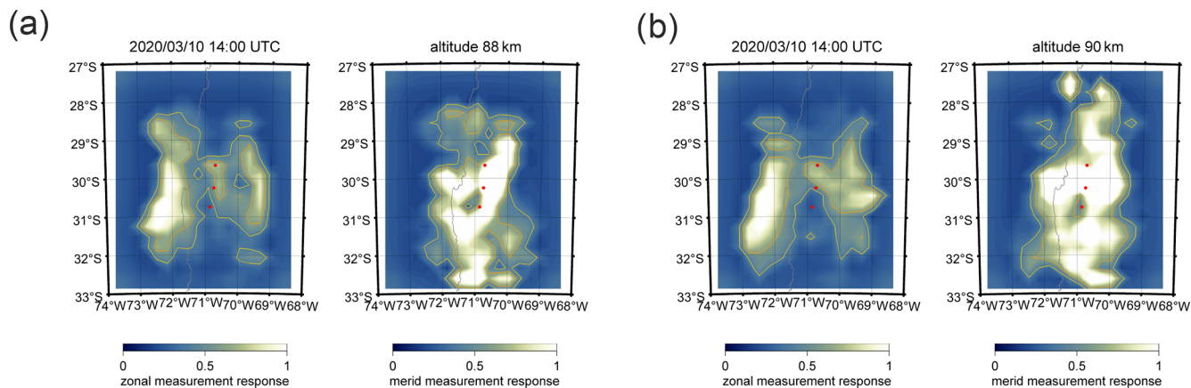
Figure 8. The four panels show the measurement response for the zonal and meridional wind components and both altitudes of the body force event above CONDOR.
