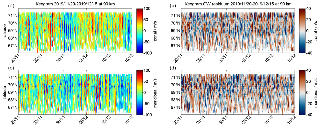
Figure 12. The four panels show color-coded latitudinal keograms of zonal and meridional winds for 22° longitude and 90 km altitude from 20 November to 15 December 2019.
