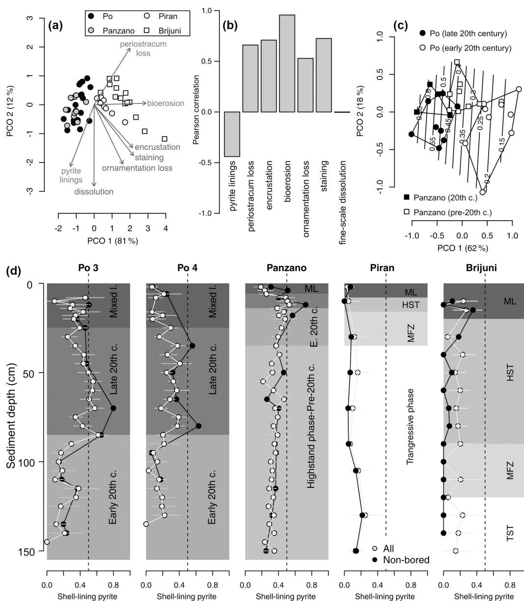
Figure 13. (a) Principal coordinate analysis (PCO) based on V. gibba alteration (using seven variables) in increments from all sites (excluding increments from the mixed layer). (b) Correlations between PCO axis 1 and seven alteration variables show that pyrite varies inversely with other alteration variables. (c) Principal coordinate analysis of increments at Po and Panzano, showing the separation between the latest HST (white circles) and the late 20th century increments (black circles), mainly determined by the frequencies of pyrite-lined specimens (contours). (d) Stratigraphic changes in the frequencies of all pyrite-lined valves (gray circles) of V. gibba peak at 40%–50% in the upper part of cores at Po 3 and Po 4 and at 50% at ~10–20 cm at Panzano. The frequencies of pyrite-lined valves are typically less than 20% at Piran and Brijuni where sedimentation rates are slow. The frequencies of pyrite-lined valves at Piran and Brijuni further decline when the frequencies of pyrite-lined valves are limited to valves not affected by bioerosion (black circles), magnifying the contrast between well-preserved pyrite-lined valves at sites with high sedimentation (primary linings) and variably preserved pyrite-lined valves at sites with slow sedimentation (with some pyrite corresponding to secondary linings).
