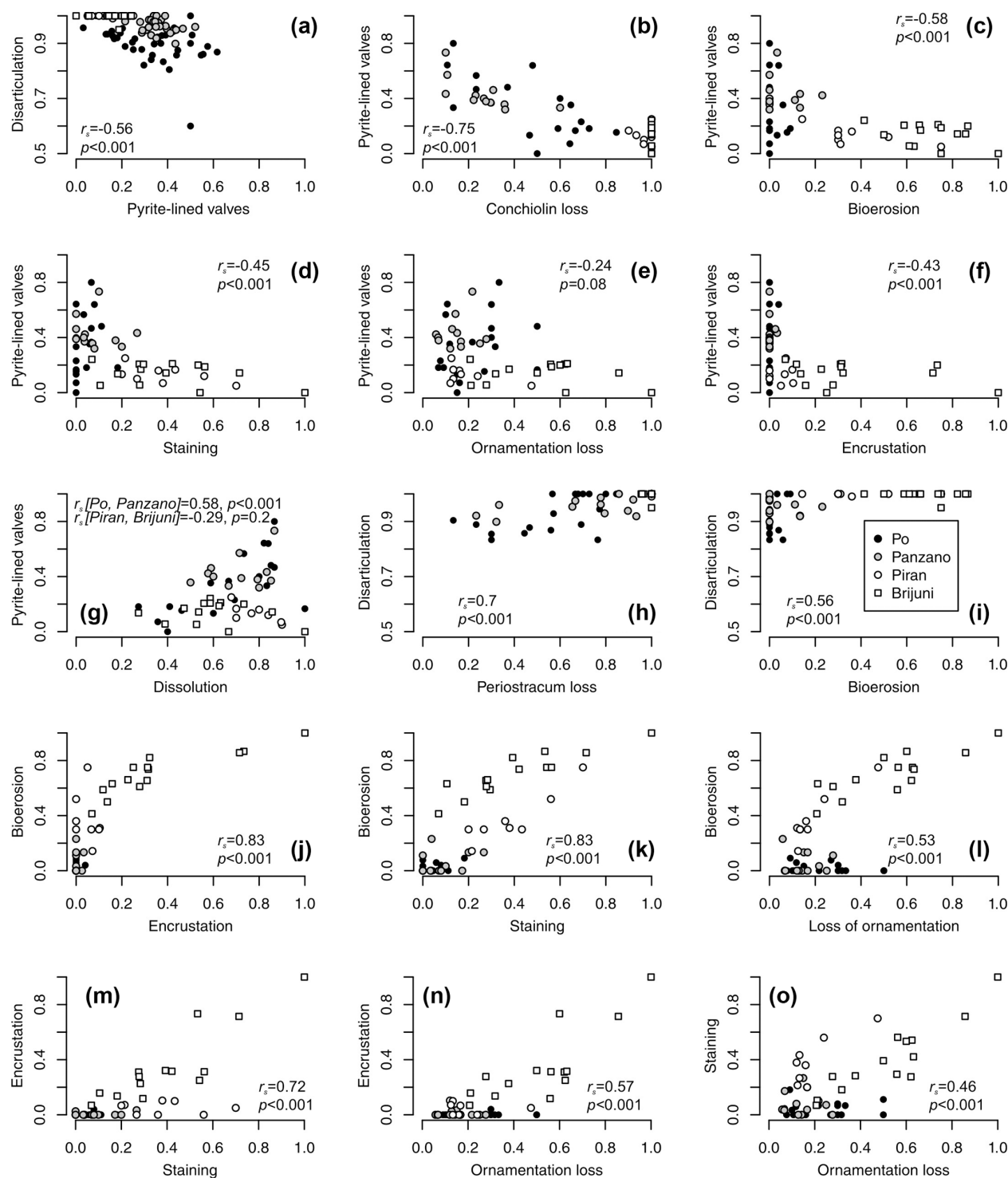
Figure 12. (a–f) Negative relationships between per-increment frequencies of pyrite-lined valves and frequencies of other types of alteration ( r_s values refer to Spearman rank correlations). (g) The relation between frequencies of pyrite-lined valves and fine-scale dissolution depends on the site location and the pathway that ultimately leads to dissolution (pyrite oxidation at Po and Panzano or bioerosion at other sites). Valves with pyrite commonly show internal fine-scale dissolution but are still associated with some surviving portions of periostracum or the conchiolin layer. However, high frequencies of dissolved specimens are associated with low pyrite preservation as specimens from Piran and Brijuni are bored and dissolved but rarely associated with pyrite grains. (h–l) Pairwise positive relationships between frequencies of disarticulation, conchiolin loss, bioerosion, encrustation, staining, and loss of ornamentation. (m–o) Pairwise positive relationships between frequencies of encrustation, staining, and ornamentation loss.
