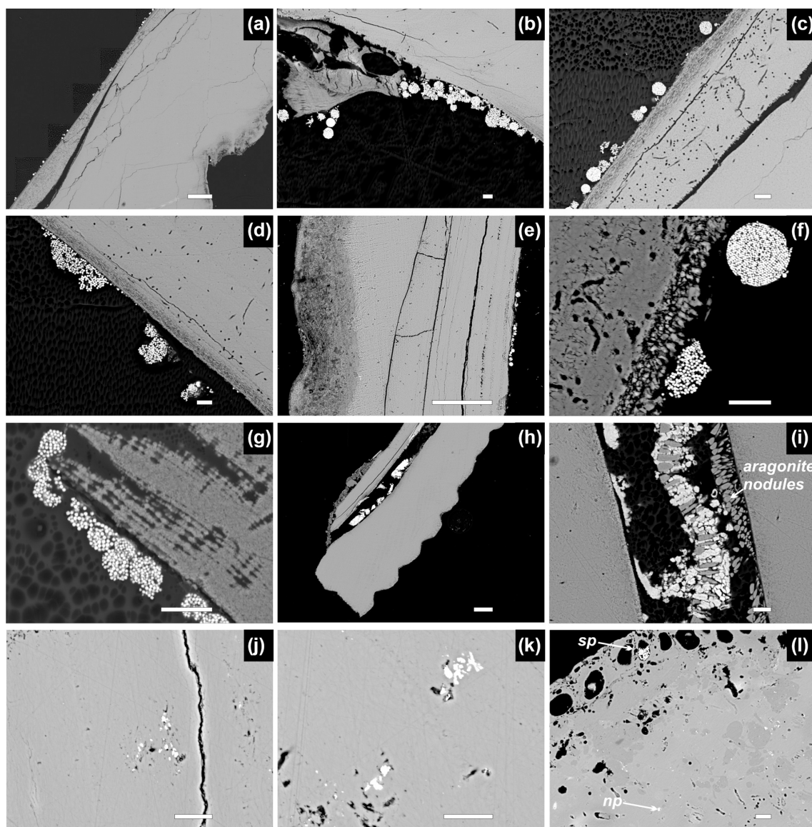
Figure 8. Backscattered electron images showing pyrite framboids on V. gibba valve interiors and in the main conchiolin layer in well-preserved valves and pyrite framboids and nanopyrite in microborings or microfractures in highly altered valves. (a–d) Pyrite framboids attached to the interior surface, Po 3 (M14)–40–45 cm. (e–f) Pyrite framboids attached to the interior surface, Po 4 (M21)–90–95 cm. (g–i) Pyrite framboids on the interior and framboids (located between aragonite nodules) rimmed by Fe oxides in the main conchiolin layer, Po 4 (M20)–120–125 cm. (j–k) A well-preserved specimen without microborings but with blueish staining containing nanopyritic inclusions (aggregation of micro-sized microcrystals), Piran (M53)–100–105 cm-1. (l) A dark-stained specimen with intense microborings, encrustations, and cementation of pores and borings filled by framboids (sp – secondary pyrite lining), by nanopyritic inclusions (np) and by high-Mg calcite (darker infills), Brijuni (M44)–140–145 cm-2. Scale bars: (e, e, h) 100 \mu m, and (b–d, f, g, i–l) 10 \mu m.
