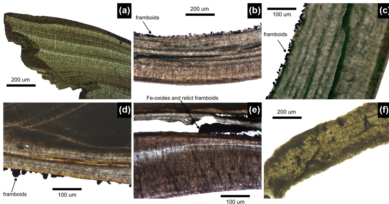
Figure 7. Thin-section photographs showing pyrite framboids on the inner surface of V. gibba and preservation of more altered valves. (a) A pristine right valve not lined by pyrite framboids, M13-65-79 cm-29. (b–c) Internal surface of well-preserved right valve lined by pyrite framboids (arrows), M21-90-95 cm. (d) Internal surface of well-preserved right valve lined by pyrite framboids, M14-40-45 cm. (e) Internal conchiolin layer within the right valve, with a dark mixture of carbonate nodules and pyrite rimmed and replaced by Fe oxides, M20-120-125 cm. (f) Strongly bored valve filled with micrite and stained by nanopartic inclusions, M44-140-145 cm.
