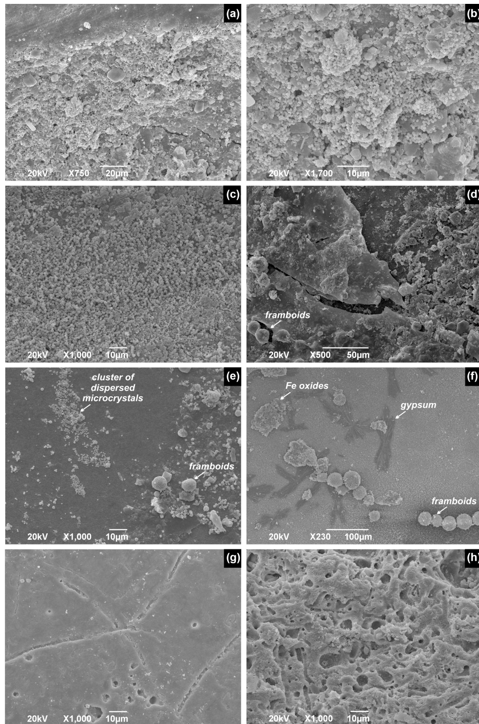
Figure 9. Internal surfaces of V. gibba with isolated and clustered framboids on well-preserved valves from Po and with intense borings on valves from Brijuni. (a–b) Dispersed pyrite microcrystals and isolated framboids clustered around the groove at which the internal conchiolin crops out. (c) Dispersed pyrite microcrystals close to the groove. (d) Sheets of organics underlain by framboids on the interior of the right valve close to the ventral margin. (e) Clusters of dispersed microcrystals and isolated framboids on the well-preserved ventral valve margin. (f) Strings of pyrite framboids, irregular flakes of Fe oxides, and small gypsum crystals. Moderate (g) and strong (h) bioerosion. (a–b) Po4-30-35 cm-28. (d–f) Po4-30-35 cm-28. (g) Brijuni-M44-70-75 cm-3. (h) Brijuni-M44-70-75 cm-1.
