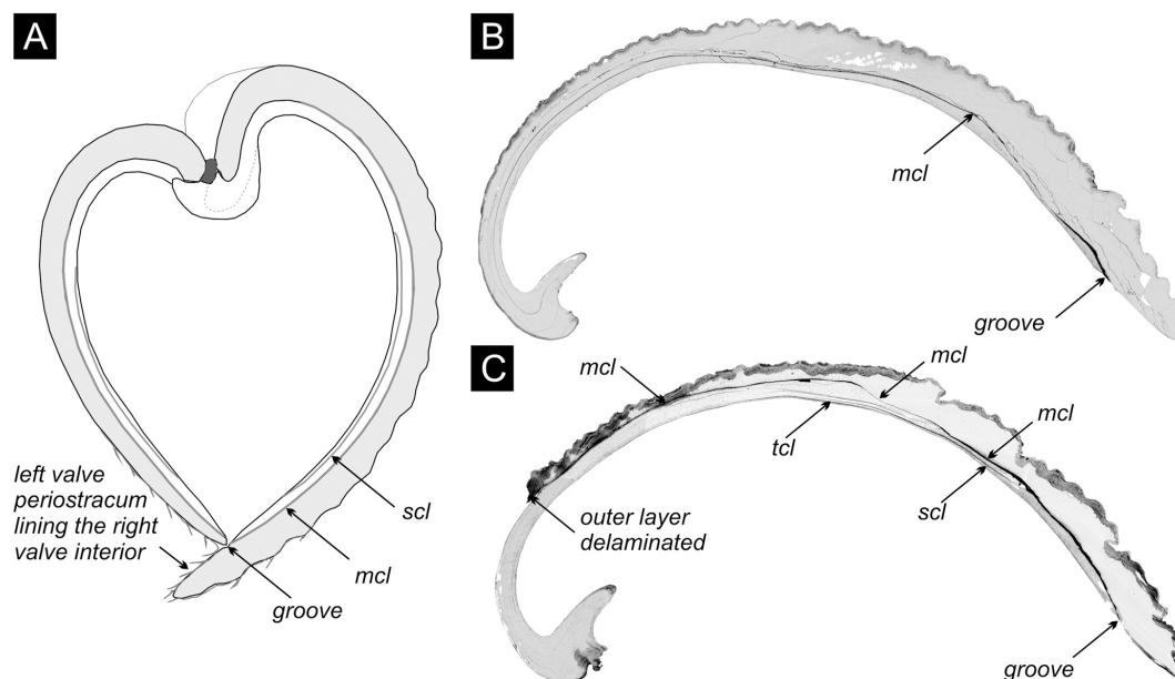
Figure 4. (a) The cross section of the articulated shell of V. gibba , adapted from Lewy and Samtleben (1979), shows that the internal conchiolin layer (mcl) separates both valves into an inner and an outer layer, and the inner layer can contain another secondary conchiolin layer (scl). The left valve fits into a groove with the conchiolin layer on the interior of the right valve. Periostracum on the left valve extends beyond its length and covers the interior of the right valve. (b) The section through the right valve with a 10–100 \mu\text{m} thick cavity (in black) initially filled by the single (main) conchiolin layer. Po 3 (core M14) at 40–45 cm. (c) The section through the right valve with 10–100 \mu\text{m} thick cavities present within the main and other conchiolin layers (mcl – main conchiolin layer, scl – secondary conchiolin layer, tcl – tertiary conchiolin layer). Po 3 (core M13) at 65–70 cm.
