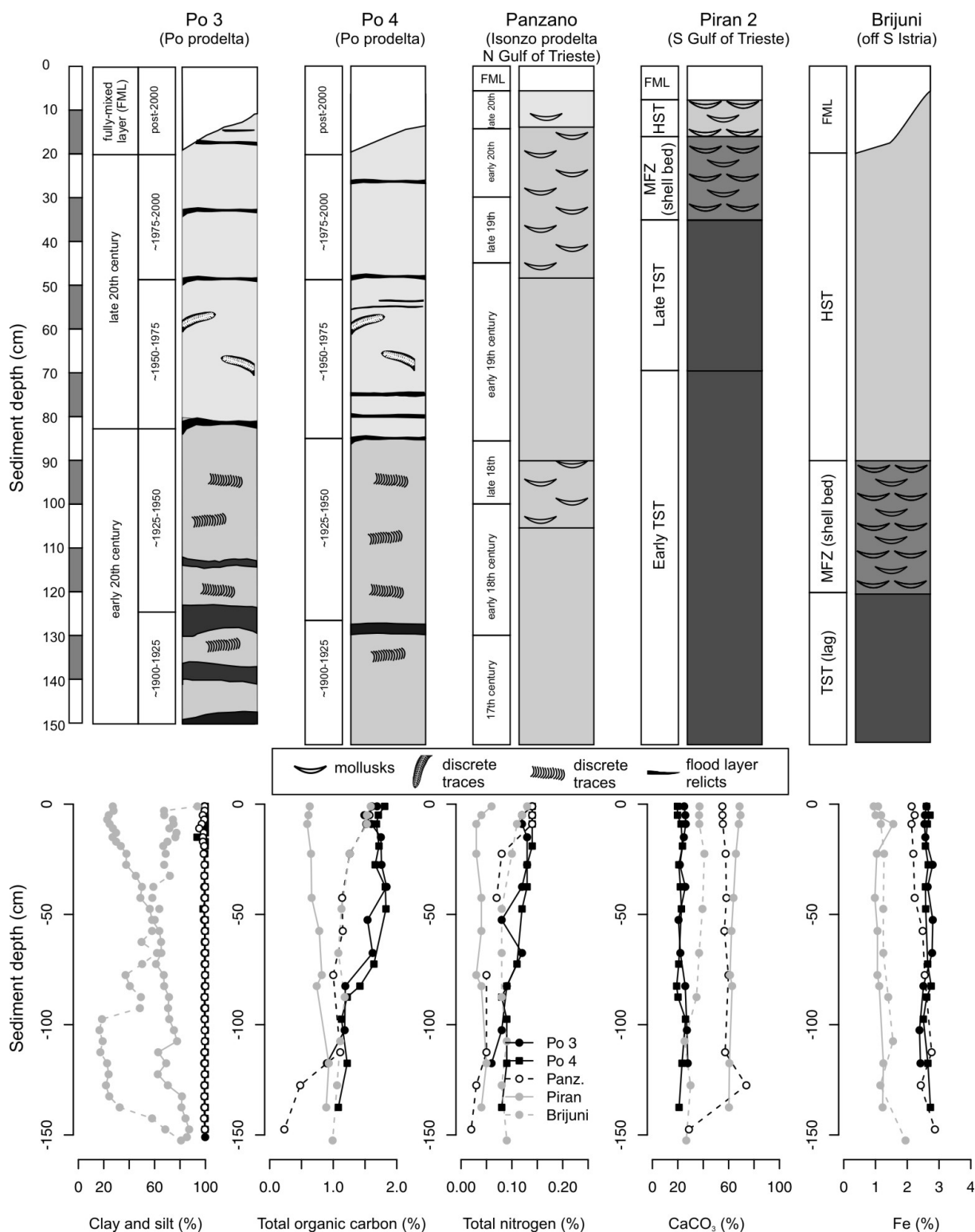
Figure 2. Top row: lithologic sections through sediment cores at five locations, with the highest sedimentation rate (1–2 cm yr -1 ) at the Po sites, intermediate net sedimentation rate (0.2–0.4 cm yr -1 ) in the Bay of Panzano, and very slow sedimentation rate at Piran and Brijuni (~0.01 cm yr -1 ), with chronostratigraphic and sequence stratigraphic subdivisions. TST – transgressive system tract, MFZ – maximum flooding zone, HST – highstand system tract, FML – fully mixed layer (its thickness varies within cores depending on differences between the estimates based on 210 Pb profiles and downcore changes in median shell age). Bottom row: stratigraphic trends in grain size, in the weight percent of total organic carbon (TOC), total nitrogen (TN), CaCO 3 (based on total inorganic carbon), and iron also discriminate between sites with higher sedimentation (Po and Panzano) and sites with slower sedimentation (Piran and Brijuni).
