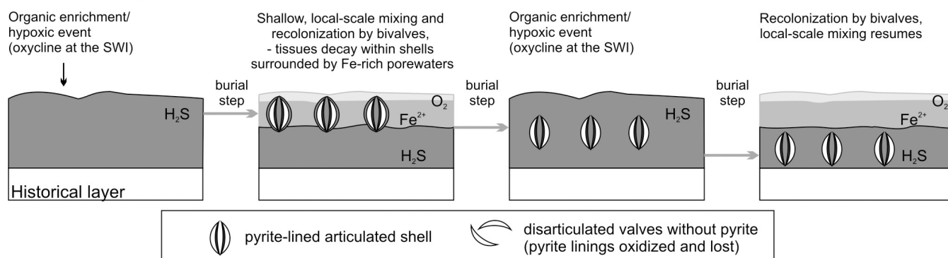
Figure 16. Two pathways characterized by differences in the frequency of hypoxic events (leading to the local extinction of infaunal organisms) and by differences in recovery rate of infaunal communities with high irrigation potential. As bivalves colonize and die at shallow sediment zones, both pathways promote the initial formation of reduced pockets, surrounded by iron-rich porewaters induced by local-scale mixing during the early recovery phase. (a) In the aftermath of hypoxia, pyrite linings in reduced pockets are formed initially in mixed sediments, but these are recycled under later recovery of irrigating organisms that oxidize deeper sediment zones and contribute to disintegration of initially articulated shells. (b) If the frequency of hypoxic events is high, the oxycline can remain permanently shallow because the recovery of infauna with high bioirrigation potential remains patchy, and some subset of shells with pyrite linings is thus not oxidized. Therefore, shells with pyrite linings can escape from the mixed layer into the subsurface stratigraphic record in (b) . In the historical layer, valves permanently remain in reducing conditions.
