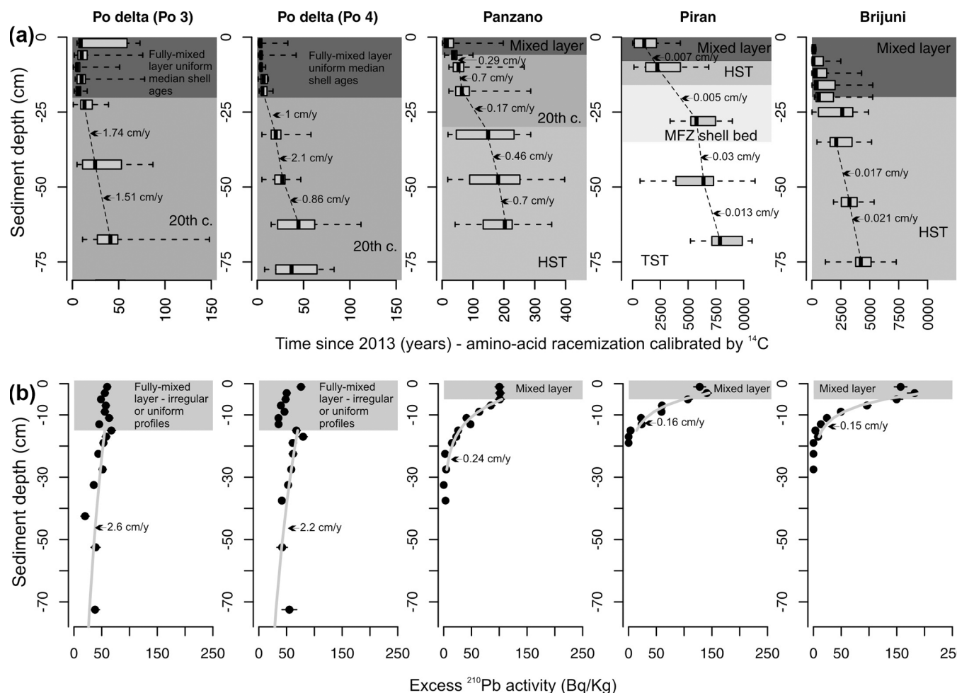
Figure 3. Downcore changes in shell ages (a) and the excess in ^{210}\text{Pb} profiles (b) that form the basis for inferences about the depth of the mixed layer (absence of downcore changes in median shell age in the uppermost parts of cores and irregular or uniform segments of the ^{210}\text{Pb} excess) and the sedimentation rate (thickness deposited over a duration defined by differences in median ages and the slope of the ^{210}\text{Pb} segments below the mixed layer in gray). We note that some variability in these estimates is also affected by bioturbation when the thickness of sediments over which the deposition is measured is too low relative to the thickness of the mixed layer, leading to overestimation of the sedimentation rate.
