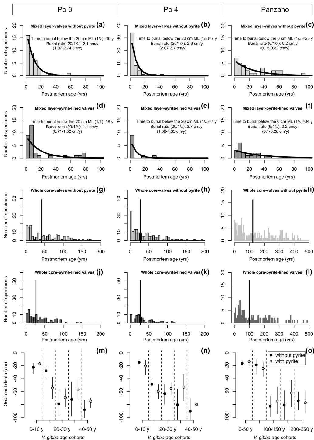
Figure 10. (a–l) Mixed-layer (a–f) and whole-core distributions (g–l) of postmortem ages of V. gibba from Po 3, Po 4, and Panzano with valves with and without pyrite showing that first, even the youngest valves less than 5–10 years old have pyritic linings. Second, the mixed-layer distributions of valves with and without pyrite show similar right-skewed shapes well-fitted by a simple exponential model (black lines) that indicates that both types of valves are buried below the mixed layer at a similar rate (burial rate corresponds to inverse of the mean age of the distribution, with 95 % confidence intervals in parentheses). The burial rate estimated on this basis is congruent with downcore changes both in median shells ages and in ^{210}\text{Pb} -based estimates of sedimentation rate at Po and Panzano, indicating that the steepness of mixed-layer age distributions primarily corresponds to burial rates. At the scale of whole cores (g–l), pyrite-lined valves exhibit a mode at \sim 25 years at Po 4 and a mode at \sim 50 years at Panzano. (m–o) Mean sediment depths of valves with (gray) and without pyrite (black) of the same age are similar. Both age and depth distributions indicate a scenario in which pyrite formation is not associated with deeper burial and occurs in reduced microenvironments in near-surface sediment zones.
