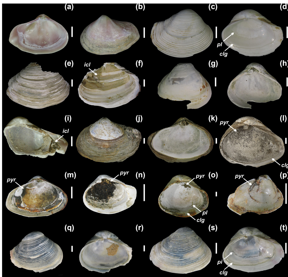
Figure 5. Varicorbula gibba from Po and Panzano (characterized by high sedimentation rates), showing the variability in external and internal preservation, with well-preserved valves with (a–b) or without periostracum (c–d) and with relicts of the main conchiolin layer (e–f). The interiors of some specimens are lined by pyritic framboids that form isolated and dispersed framboids (k), strings (l), and patchy or continuous coatings on the conchiolin layer (m–p). These specimens tend to be associated with brownish grains and streaks and with internal surface dissolution. Some specimens have a blueish color (q–t). (a–b) Left valve, M28-65-70 cm-29. (c–d) Right valve, M21-90-95 cm-1. (e–f) Outer layer of the right valve, M13-65-70 cm-25. (g–h) Inner layer of the right valve, M13-20-25 cm-8. (i) Internal conchiolin layer exposed in a fragment, M20-120-125 cm. (j–k) Left valve with periostracum and finely dispersed pyrite framboids on interior, M21-2-4 cm-2. (l) Interior of the right valve with strings of pyrite framboids, M21-90-95 cm. (m) Interior of the left valve lined by pyrite framboids, M28-110-115 cm-22. (n) Interior of the right valve almost continuously lined by pyrite framboids, M28-110-115 cm-14. (o) Interior of the right valve lined by patches of pyrite framboids, M21-30-35 cm-29. (p) Interior of the left valve with strings of oxidized pyrite framboids, M28-125-130 cm-21. (q–r) Blue-stained right valve, M28-85-90 cm-1. (s–t) Blue-stained right valve, M21-105-110 cm-4. Note: clg – conchiolin groove, pl – pallial line, pyr – framboidal pyrite, icl – internal conchiolin layer. Scale bar: 1 mm.
