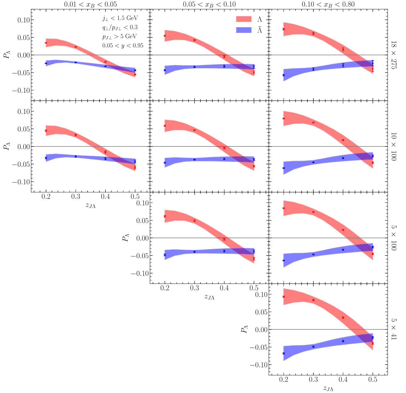
FIG. 14. Our projections for spontaneous \Lambda polarization. The red band and blue bands represent our theoretical uncertainty using the parameters obtained from the baseline fit in Sec. IV B for \Lambda and \bar{\Lambda} production, respectively. The error bars represent our projected statistical uncertainties at an integrated luminosity of 100 \text{ fb}^{-1} . To obtain these results, we integrate over the kinematic regions listed in the top right of the left plot. Furthermore, we also impose the conditions that x_B is within each of the listed regions.
