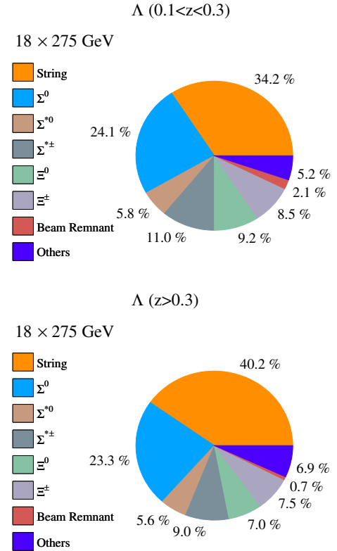
FIG. 5. Origins of \Lambda for 0.1 < z < 0.3 and z > 0.3 according to the event records provided by the PYTHIA event generator for the 18 \times 275 \text{ GeV}^2 energy configuration.
