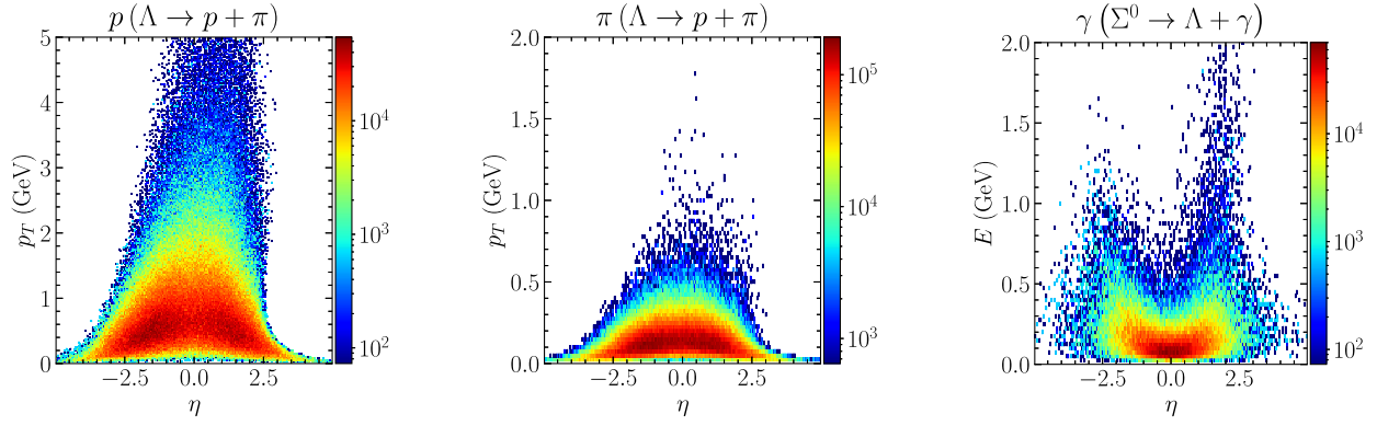
FIG. 3. Final state particle distributions in transverse momentum (energy) and pseudorapidity space for proton (left), pion (middle), and photon from \Sigma^0 decay (right). Here we display the results at the collision energy 18 \times 275 \text{ GeV}^2 and we note that the distributions for other energy configurations are similar.
