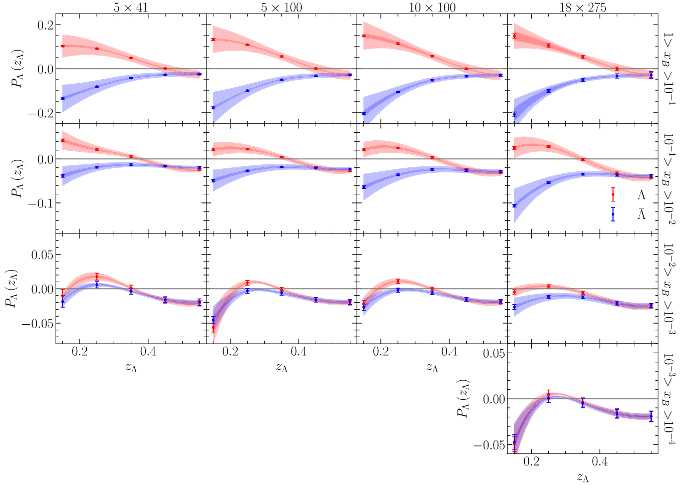
FIG. 9. Theoretical predictions are compared against the pseudodata generated in the reweighting method at 40 fb -1 . The rows are grouped by the range of x_B while the columns are group by the energy configuration of the collision where the first number represents the energy of the lepton beam in GeV and the second number represents the energy of the hadron beam in GeV. The light band represents the theoretical uncertainty from the baseline fit to the Belle data while the dark band represents the theoretical uncertainty from the fit including the pseudodata.
