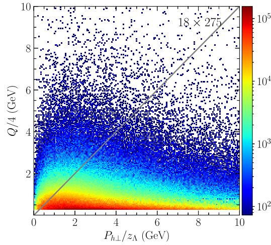
FIG. 4. Illustration of the impact of the constraint P_{h\perp}/z_\Lambda < Q/4 . Only events above the line are accepted. The efficiency of this cut depends on the hard scale Q^2 and is approximately 7% for Q^2 > 1 \text{ GeV}^2 , 25% for Q^2 > 10 \text{ GeV}^2 and 50% for Q^2 > 100 \text{ GeV}^2 . Here, we provide the result for the 18 \times 275 \text{ GeV}^2 energy configuration while we note that the results for the other collision energies configurations are similar.
