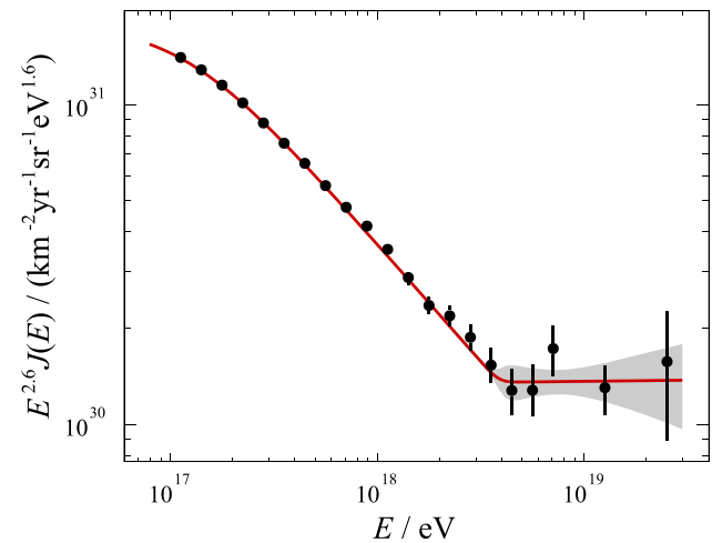
Fig. 13 Unfolded energy spectrum of the SD-750, scaled by E^{2.6}
