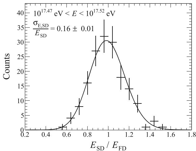
Fig. 8 An example of the ratio of the energy assignments for the SD and FD is shown with black crosses for the energy bin indicated in the plot. The best fit ratio distribution for this bin is shown by the black line
