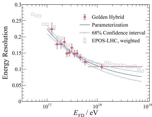
Fig. 9 The total SD energy resolution, as calculated using the golden hybrid events (red circles) is shown in bins with equal statistics. The parameterization of the resolution is shown by the solid blue line and the corresponding 68% confidence interval in dashed lines. The energy resolution, calculated using mass-weighted MC air showers (gray squares), is shown as a verification of the method
