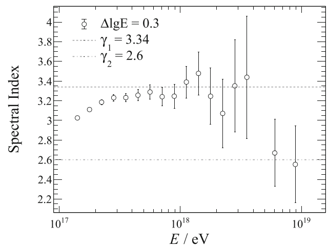
Fig. 14 Evolution of the spectral index with energy. The measured spectral points were fit to power laws within a sliding window of \Delta \lg E = 0.3 . The values of \gamma_1 and \gamma_2 are represented by the dashed and dash-dotted lines, for reference
