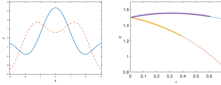
Fig. 1 Left: Example profiles from the FPI, (14), with \varepsilon = 0.01 (the profile on branch with \beta = 1/\sqrt{2} , (12), is the solid curve, the profile on the branch with \beta = -1/\sqrt{2} is the dashed curve). Right: The speed–amplitude curves for two branches of ripples in the Akers–Milewski equation are depicted. The output of the FPI (triangles) is compared to that of the quasi –Newton iteration (solid lines).
