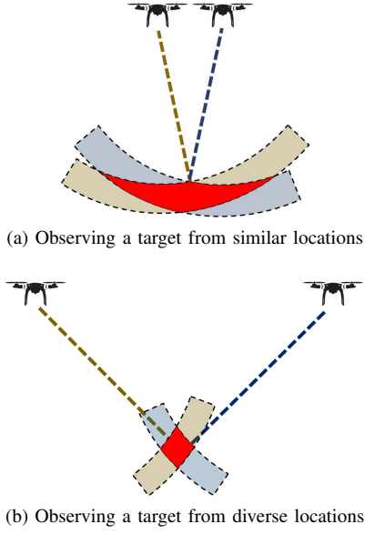
Fig. 2: Two target-to-drone range sensing drones
