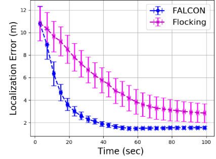
(b) Localization error vs. time
