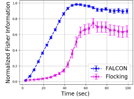
(a) Normalized FI vs. time
