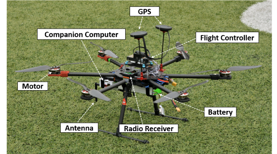
Fig. 3: FALCON drone platform
