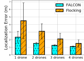
Fig. 15: Localization accuracy as the number of drones increase in the network
