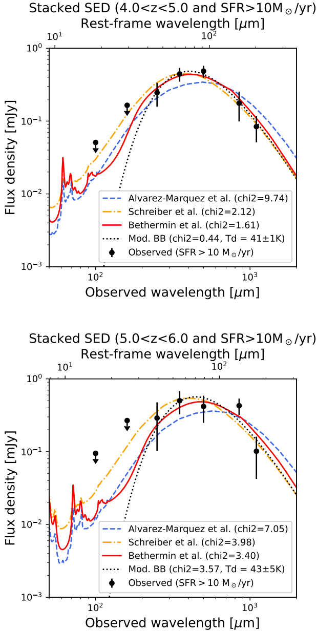
Fig. 9. Comparison between the Álvarez-Márquez et al. (2016 , blue dashed line), Schreiber et al. (2018 , orange dot-dashed line), and Bethermin et al. (2017 , red solid line) IR SED templates and the observed mean SEDs of SFR > 10 M_{\odot} \text{ yr}^{-1} galaxies measured by stacking (black dots, see Sect. 4.2). The black dotted line is the best fit of the \lambda_{\text{rest-frame}} > 40 \mu\text{m} data points by a modified blackbody with \beta fixed to 1.8 (the temperature in the legend is provided in the rest frame). Upper and lower panels: 4 < z < 5 and 5 < z < 6 , respectively.
