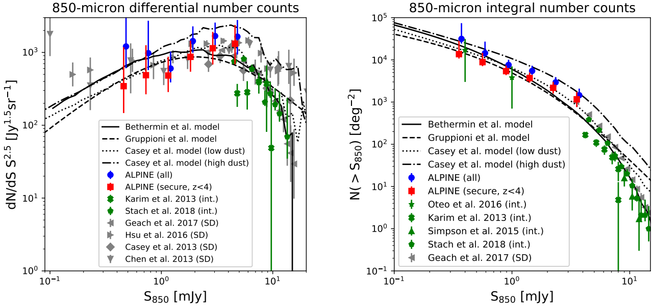
Fig. 13. Left panel: differential number counts at 850 \mu\text{m} . The blue circles are the counts derived from the full ALPINE nontarget sample. The red squares are computed from the ALPINE nontarget sources with a confirmed optical or near-IR counterpart below z = 4 (secure z < 4 sample). It is thus a secure lower limit, since sources clustered with ALPINE sources are excluded. The green crosses and pentagons are the interferometric measurements of Karim et al. (2013) and Stach et al. (2018) , respectively. The gray left-facing triangles, right-facing triangles, diamonds, and down-facing triangles are the measurements performed using single-dish data with a lower angular resolution by Geach et al. (2017) , Hsu et al. (2016) , Casey et al. (2013) , and Chen et al. (2013) , respectively. The solid, dashed, dotted, and dash-dot lines are the models of Bethermin et al. (2017, SIDES simulation) , Gruppioni et al. (2011) , Casey et al. (2018, low dust) , and Casey et al. (2018, high dust) . Right panel: integral number counts at 850 \mu\text{m} . The symbols are the same as in the left panel. The interferometric measurements of Oteo et al. (2016) and Simpson et al. (2015) , respectively, are represented by green stars and triangles.
