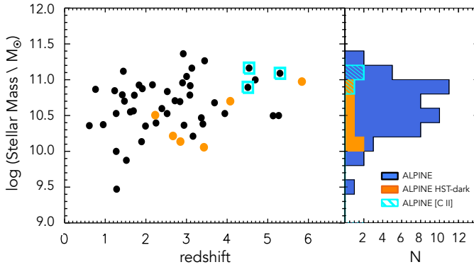
Fig. 9. Stellar mass versus redshift (left) and stellar mass histogram (right) for ALPINE continuum non-target detections. The black filled circles and blue filled histogram show the distribution of the whole sample, while the orange circles and histogram show the locus occupied by the HST+near-IR dark sources. The cyan open squares and dashed-histogram show, for comparison, the locus of the sources identified with [C II] emitters at the same redshift of the ALPINE targets (we note that the two without photometric counterparts are missing, since for them a mass estimate was impossible).
