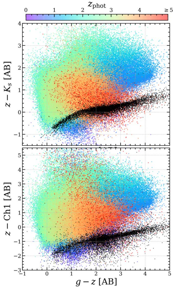
Figure 12. Color–color diagrams showing stars (black) and galaxies (colored by z_{\text{phot}} ) classified by LePhare for THE FARMER photometry, shown in gK_s (top) and gzch1 (bottom) color–color diagrams. For simplicity, galaxies with z_{\text{phot}} > 5 are shown also by red points. Only sources with S/N > 3 in g , z , K_s , and ch1 in the UltraVISTA area outside the HSC bright-star halos are shown.
