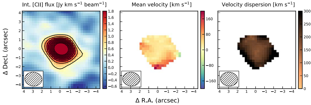
Figure 25. Moment maps of the [\text{C II}]_{158\ \mu\text{m}} emission. The integrated velocity and velocity dispersion are only shown in pixels at the 3\sigma level. The absence of any velocity structure is expected, given that the 3\sigma detected area covers only \sim 4 beams.
