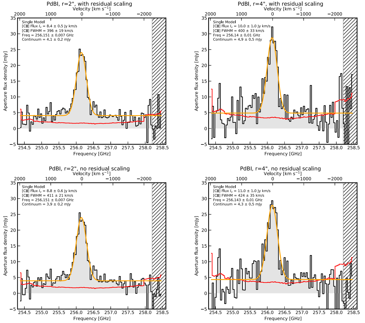
Figure 20. The total spectra of the [\text{C II}]_{158 \mu\text{m}} line, with (first row) and without (second row) residual scaling, extracted in r = 2'' and r = 4'' apertures (the first and second columns, respectively), in the PdBI data. The single-Gaussian (+continuum) fits to both data sets are shown in orange. In the absence of residual scaling, the continuum flux drops away from the [\text{C II}]_{158 \mu\text{m}} line in the larger apertures (see the text for details). Even though no continuum was subtracted in the UV plane, the continuum flux approaches \sim 0 mJy at the band edges in the r = 4'' aperture (without residual scaling), creating the illusion of a broad emission line.
