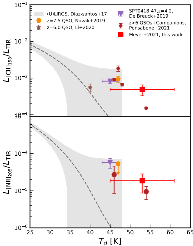
Figure 9. [\text{C II}]_{158\ \mu\text{m}} and [\text{N II}]_{205\ \mu\text{m}} line deficits of local (U)LIRGS (shaded gray; Díaz-Santos et al. 2017), the high-redshift galaxy SPT0418-47 (the purple triangle; De Breuck et al. 2019), and high-redshift quasars (the orange pentagon, dark orange star, and dark red circles; Novak et al. 2019; Li et al. 2020; Pensabene et al. 2021, respectively) and companion galaxies (the dark red circles; Pensabene et al. 2021). Our measurements for J1148+5251 are shown via the red squares.
