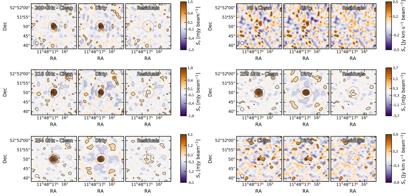
Figure 14. Clean, dirty, and residual maps for a Högbom clean to 2\sigma of the 200 GHz continuum, [N II] _{205\ \mu\text{m}} emission, the 216, 259, and 274 GHz continua, and finally the [O I] _{146\ \mu\text{m}} emission.
