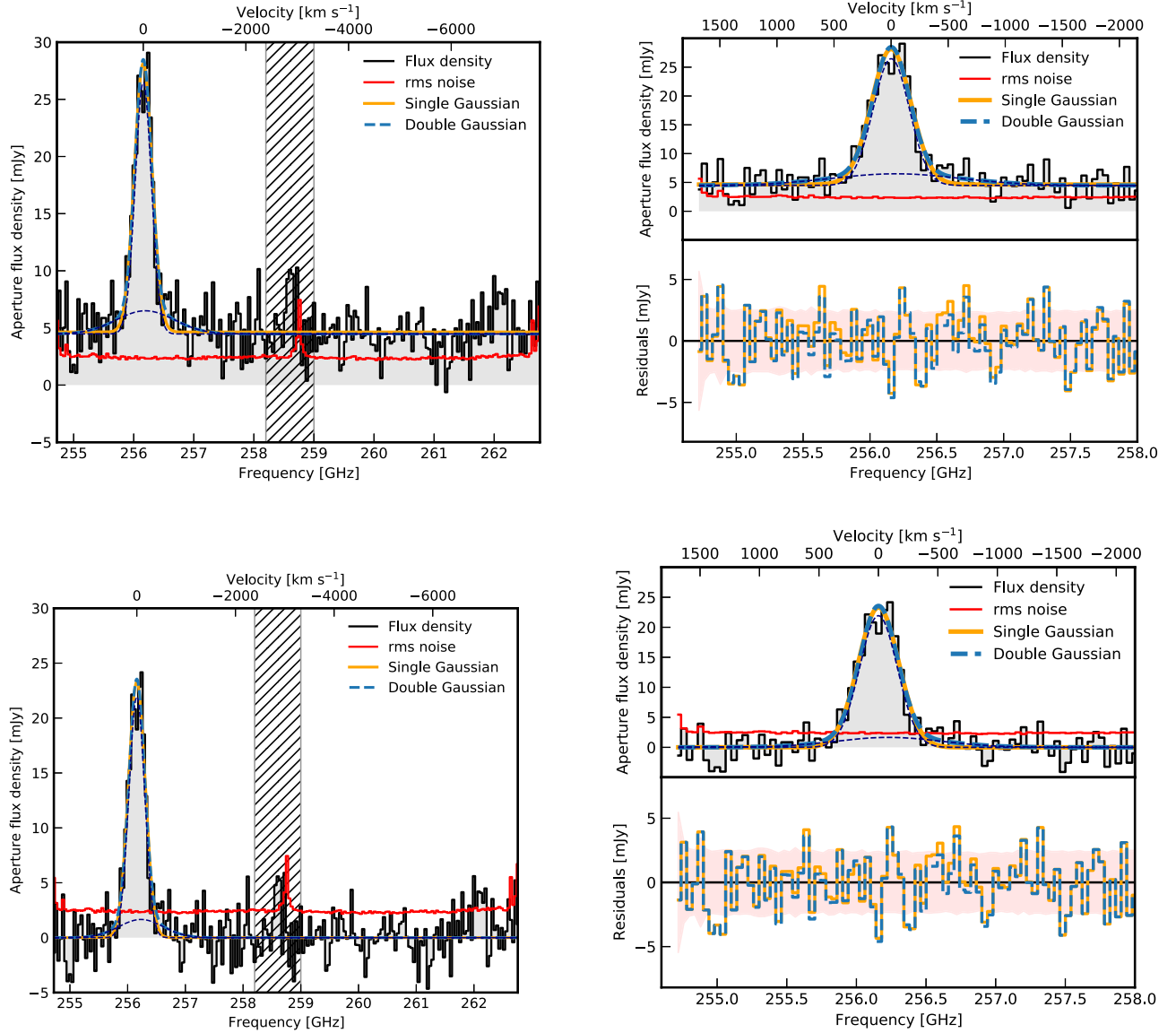
Figure 5. The total (top panels) and continuum-subtracted (bottom panels) spectra of the [\text{C II}]_{158\ \mu\text{m}} line (black), extracted in a r = 3'' aperture using residual scaling and one- and two-component Gaussian fits (the orange line and the dashed-dotted blue line, respectively). The thin dashed dark blue lines show the two components of the double-Gaussian model. Both models are fitted to the entire frequency range, with the exception of the overlap between the two sidebands that is coincident with an atmospheric absorption feature (hatched in gray) and the 262 GHz feature (see the text). The right panels show a zoomed-in version of the left plots and the residuals of the two models. The shaded red areas in the bottom of the right panels show the 1\sigma noise level, computed using the rms noise in each channel in mJy beam ^{-1} with the sigma-clipping scaled accordingly for the number of beams in the r = 3'' aperture. The median noise level at \nu_{\text{obs}} > 263 GHz is 2.36 \pm 0.14 mJy, whereas a direct rms estimate from the continuum-subtracted spectrum at the same frequencies gives 2.00 \pm 0.15 mJy. We find no evidence for a broad [\text{C II}]_{158\ \mu\text{m}} emission line in the new NOEMA data (see the text for details).
