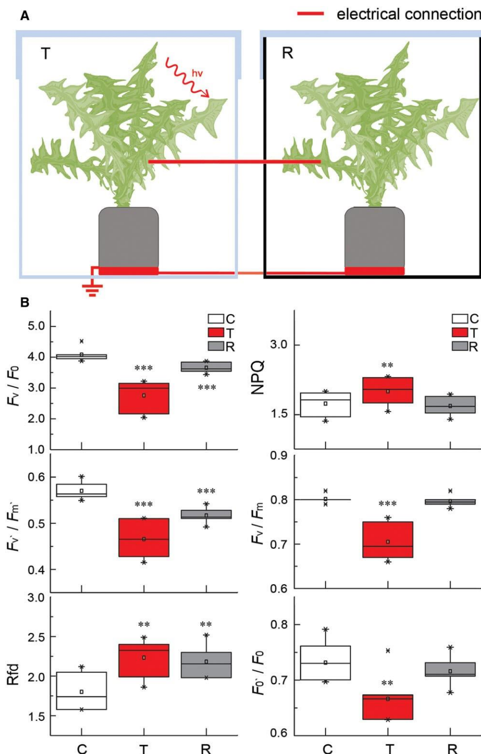
Figure 4 Changes in Chl a fluorescence in transmitter and receiver dandelion plants connected by a copper wire. A, Schematic diagram of the experiment presented in (B). Two different dandelion plants were placed on copper discs in separate plastic boxes, one of which was transparent (T, transmitter plant), while the other box had black walls (R, receiver plant). The plants and discs were coupled by copper wires threaded through the walls of the boxes. The ends of the wires coupling the plants were attached to the main vein of the leaves, and then the plants were grown for 2 days under standard laboratory conditions. Immediately prior to the experiment, the boxes were covered with lids and sealed. The T plant was stressed with a laser pointer light ( 2,000 \text{ Imol photons m}^{-2} \text{ s}^{-1} , blue 450 nm), while the R plant was untreated. B, Quantification of Chl a fluorescence parameters in C, T, and R plants: potential photosynthetic activity ( F_v/F_0 ), PSII maximum efficiency ( F_v/F_m ), Chl fluorescence decrease ratio (vitality index Rfd), NPQ, maximum quantum yield of PSII photochemistry in the dark-adapted state ( F_0/F_m ), fluorescence intensity ratio ( F_0/F_0 ). Control (C) are untreated plants before the experiment. *** P \leq 0.001 ; ** P \leq 0.01 ; * P \leq 0.05 , indicate significant differences between C and T as well as between C and R, as determined by Student's t test. Data are shown as means \pm SE ( n = 10 ). The control experiment is presented in Supplemental Figure S10.
