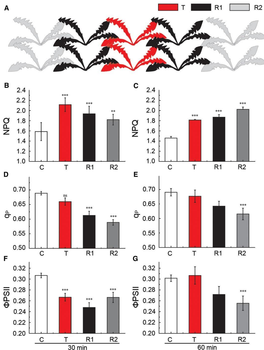
Figure 5 Changes in Chl a fluorescence in a chain of connected dandelion plants under field conditions. A, Schematic diagram of the experiments presented in B–G. Ten dandelion plants arranged in a two-chain system touching array were grown in one pot under laboratory conditions, before being moved to the field and acclimated for 1 week. Before the experiment, leaves were sprayed with water to ensure continuous contact between injured transmitter (T plants) and untreated receivers (R1 plants, primary receivers in direct contact with T; R2 plants, secondary receivers in direct contact with R1). B–G, Quantification of Chl a fluorescence parameters: NpQ, q_p , and \Phi_{PSII} . Control (C) indicates uninjured T, R1, and R2 plants. *** P \leq 0.001 ; ** P \leq 0.01 indicate significant differences between C and T as well as between C and R, as determined by Student's t test; ns, not significant. Data are shown as means \pm SE (C, n = 30 ; T, n = 6 ; R1, n = 12 ; and R2, n = 10 ). B, D, and F, Parameters measured at 30 min following injury of T. C, E, and G, Parameters measured at 60 min following injury of T.
