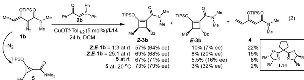
Scheme 3. Diastereoselectivity and enantioselectivity in [3 + 1]-cycloaddition reactions with \gamma -methyl enoldiazoamide 1b .
