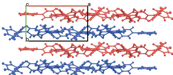
Figure 3 Crystal packing of the title compound viewed along [001]. Alternating layers are highlighted in blue and red.
