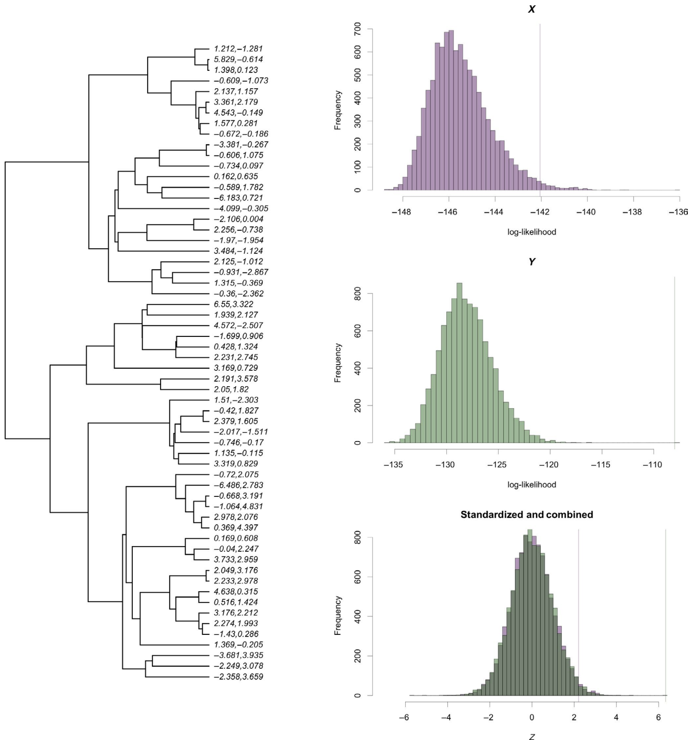
FIGURE 1 Plot of phylogenetic tree with x,y values, plus frequency histograms for the RRPP log-likelihood values for two variables, X and Y . Vertical lines indicate observed values. In the last panel, histograms have been combined for standardized values
