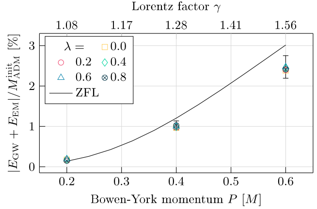
FIG. 2. Total energy lost by gravitational and electromagnetic waves normalized to the initial ADM mass. At any given Bowen-York momentum P , the energy lost for different values of \lambda is the same (within our error, see Supplemental Material [46]). The black line is the zero-frequency limit (ZFL) prediction [63] [Eq. (1) with E_{\infty} = 0.13 ], which has been shown to be accurate for uncharged collisions [3,6].
