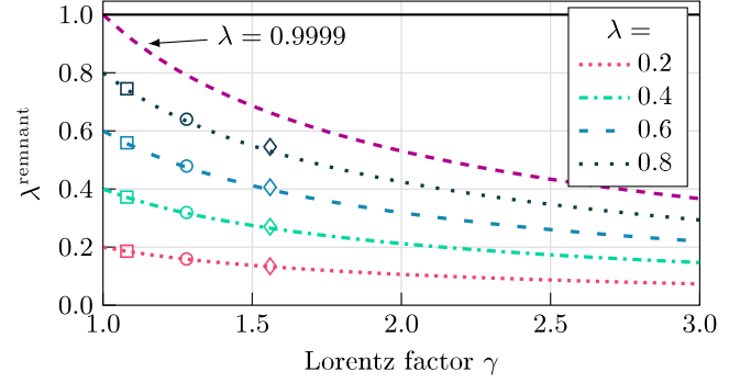
FIG. 3. Charge-to-mass ratio \lambda^{\text{remnant}} for the remnant left by a merger of two equal-mass black holes with initial Lorentz factor \gamma and charge-to-mass ratio \lambda . The curves are obtained with Eq. (3) assuming \Upsilon(\gamma) = 0 (expected from the fact that charge does not matter in the energy emitted in these mergers) and the markers are the values from our simulations. The figure seems to hint that the only case where we can obtain an overcharged remnant is with \lambda, \gamma \rightarrow 1 , where our approximations break down and previous studies found no violation [40].
