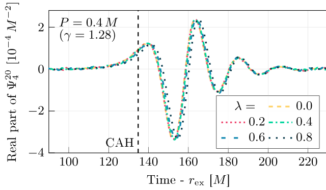
FIG. 1. Real part of the dominant multipolar component of the Newman-Penrose scalar \Psi_4 ( l = 2, m = 0 ) for simulations with different charge-to-mass ratio \lambda as extracted at radius r_{\text{ex}} = 131.430M . Note that no time shift was applied to the signals: the almost identical alignment indicates that charge has a negligible influence in these collisions. The time of formation of the horizon is also nearly insensitive to the value of charge.
