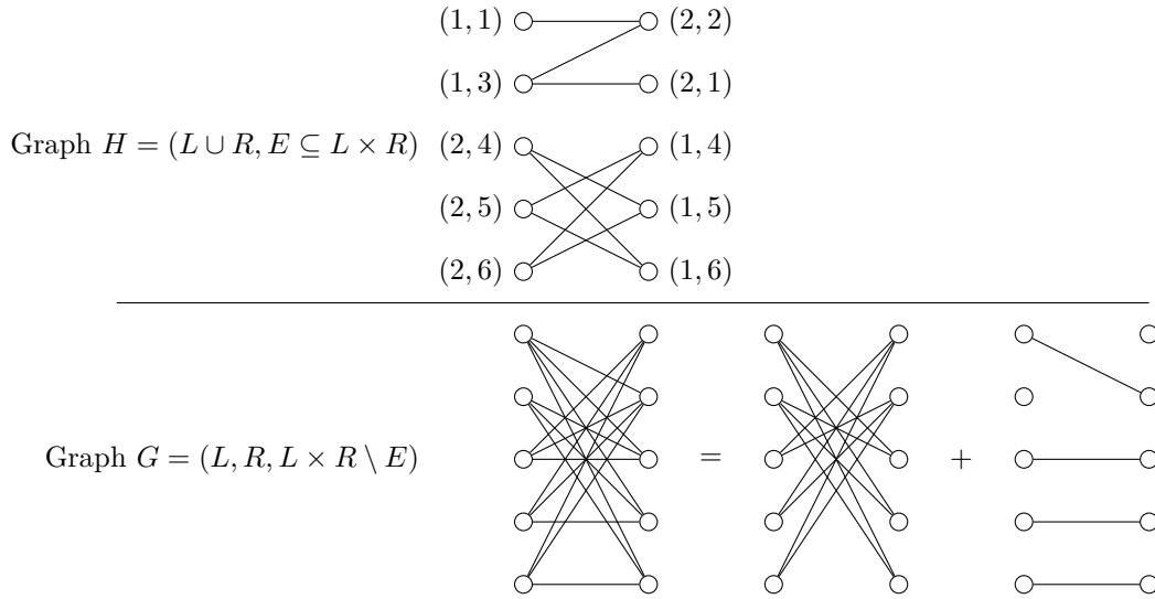
■ Figure 7 Example for the tightness of Corollary 34. Note that the loopless undirected graph H = (L \cup R, E) = P_4 + C_6 , where E \subseteq L \times R , is an induced subgraph of K_2 \times K_{\mathbb{N}} . The (partition) vertex mapping of each vertex is explicitly mentioned next to it. However, the bipartite graph G = (L, R, L \times R \setminus E) is not P_4 -free and, hence, P_4\text{-fc}(G) \geq 2 ; in fact, we have P_4\text{-fc}(G) = P_4\text{-fp}(G) = 2 . The edges of G partition into K_{2,3} + K_{3,2} and 4K_{1,1} .
