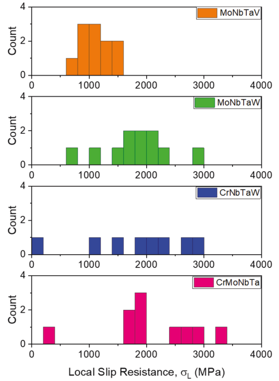
(f) {123} Screw
