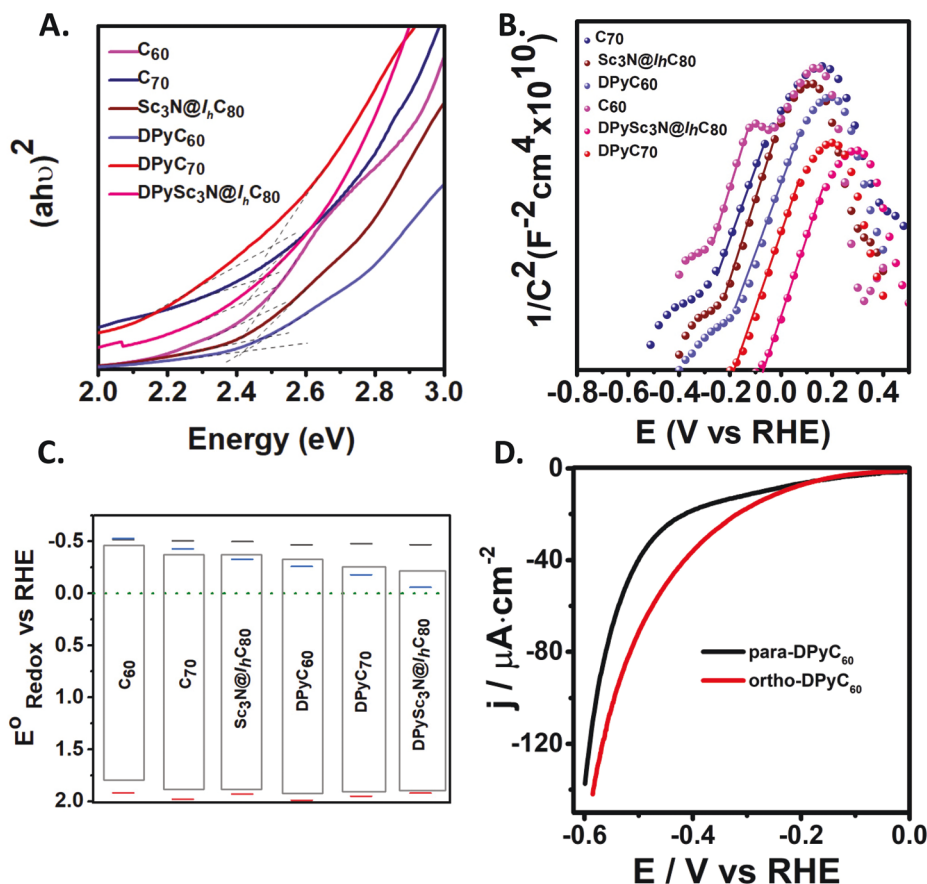
Fig. 3 (A) Tauc plots; (B) Mott-Schottky plots (capacitance values were derived from the electrochemical impedance obtained at each potential with 1 kHz frequency); (C) band gap profile; and D. LSV curves comparing para -DPyC 60 and ortho -DPyC 60 .
