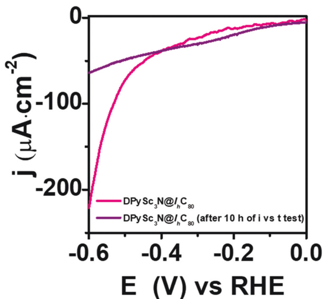
Fig. 4 Final LSV curve of the DPySc 3 N@I h C 80 of a 10 h i-t experiment.
