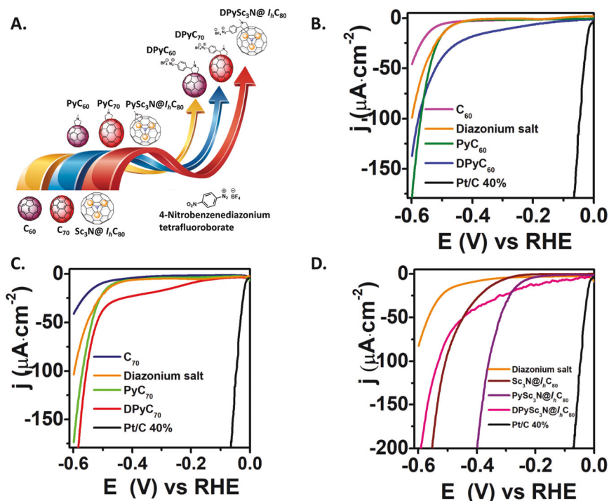
Fig. 1 (A) Summary of the compounds used in this study as controls and catalysts, (B) LSV curves for C 60 and C 60 derivatives, (C) LSV curves for C 70 and C 70 derivatives, (D) LSV curves for Sc 3 N@I h C 80 and Sc 3 N@I h C 80 derivatives.
