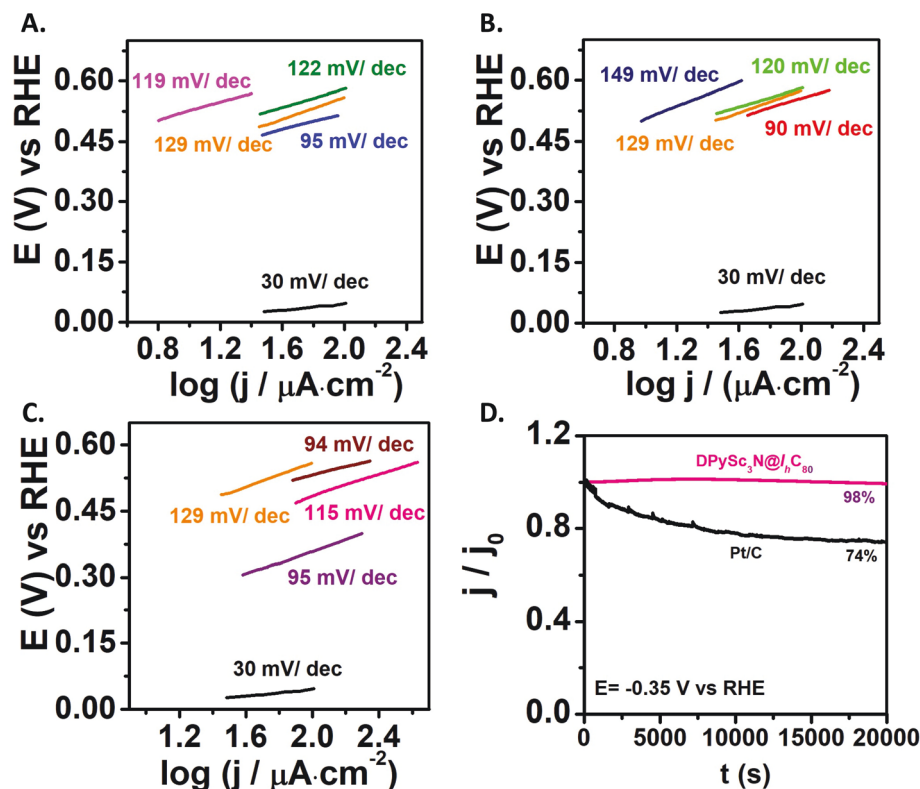
Fig. 2 Tafel plots for (A) \text{C}_{60} (magenta), \text{PyC}_{60} (green), diazonium salt (orange), \text{DPyC}_{60} (blue) and Pt/C 40% (black); (B) \text{C}_{70} (navy), \text{PyC}_{70} (light green), diazonium salt (orange), \text{DPyC}_{70} (red) and Pt/C 40% (black); (C) \text{Sc}_3\text{N}@I_h\text{C}_{80} (brown), \text{PySc}_3\text{N}@I_h\text{C}_{80} (purple), diazonium salt (orange), \text{DPySc}_3\text{N}@I_h\text{C}_{80} (pink) and Pt/C 40% (black); (D) electrochemical stability studies for the best catalyst \text{DPySc}_3\text{N}@I_h\text{C}_{80} (pink) compared to the commercially available Pt/C 40% (black).
