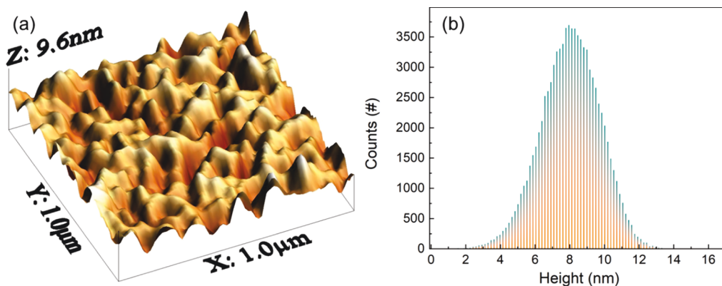
Figure 4. (a) 3D AFM image of a heteroepitaxial Nb film. (b) Surface roughness histogram of the AFM image.
