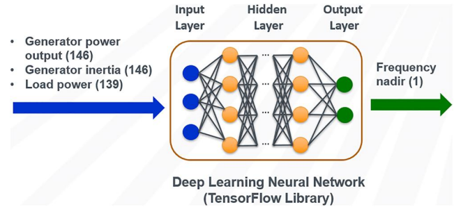
FIGURE 9 Deep learning neural network-based frequency stability assessment
