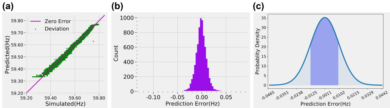
FIGURE 11 Statistic error of frequency nadir prediction. (a) Predictions on testing dataset. (b) Prediction Error histogram. (c) Prediction Error PDF
