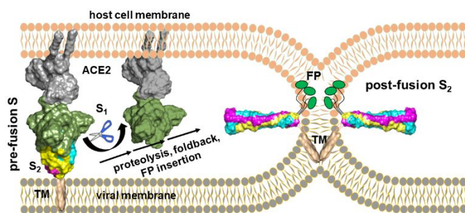
Figure 2. Transformation of prefusion S to mature S 2 at a hemi-fusion stalk. Maturation of S 2 frees FP for membrane insertion and fusion. The structures of post-fusion S 2 , ACE2, an ACE2-S complex, and the TM domain are from refs 11–14 , respectively.
