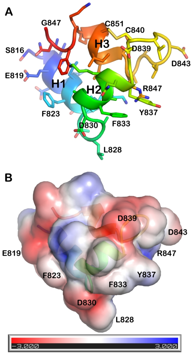
Figure 4. The fusion peptide of SARS-CoV-2 closes into a wedge-shaped structure in bicelles.
