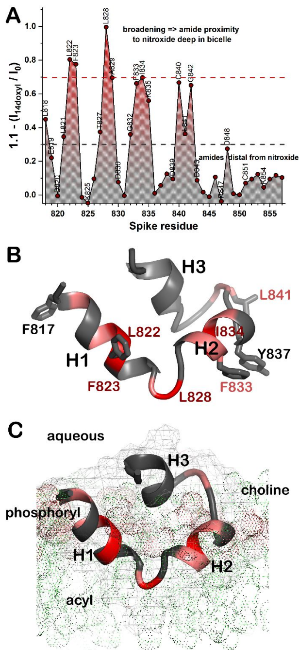
Figure 5. PRE and NOE evidence of FP insertion into bicelles. About one nitroxide spin-labeled 14-doxyl PC probe per leaflet was added to the bicelles. Proximity to the nitroxide label deep in the bicelles is symbolized with red for strong paramagnetic broadening of the amide NMR line. Gray symbolizes minimal broadening. (A) The PREs are estimated from amide NMR peak heights before and after addition of 14-doxyl PC. The ^{15}\text{N} HSQC used for detection was modified to include a ^1\text{H} PROJECT CPMG train of 8 ms 39,52 . (B) Residues with PREs to amide groups \geq 0.7 in A are
