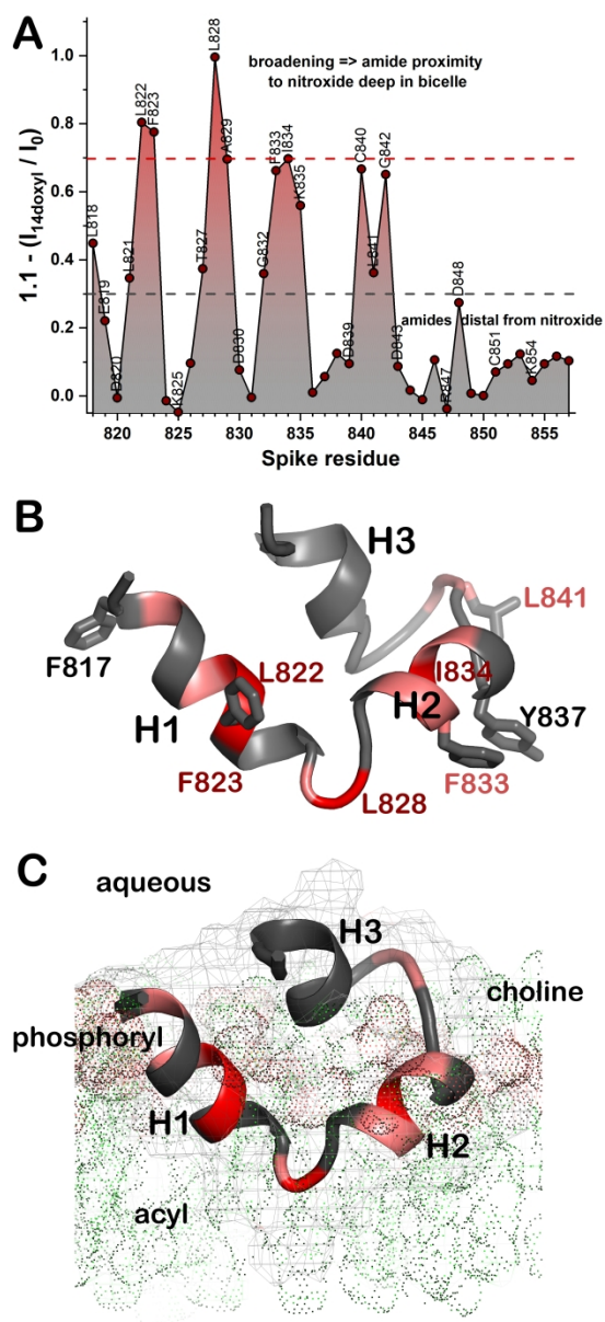
Figure 5. PRE and NOE evidence of FP insertion into bicelles.
