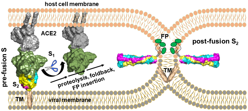
Figure 2. Transformation of prefusion S to mature S 2 at a hemi-fusion stalk.
