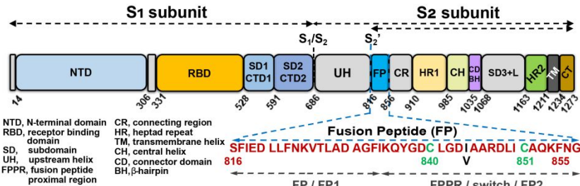
Figure 1. Subunits, domains, and fusion peptide sequence of SARS-CoV-2 Spike. The sequence of the fusion peptide (FP) of this study is shown in red. Its nomenclature in other studies is labeled with gray text.
