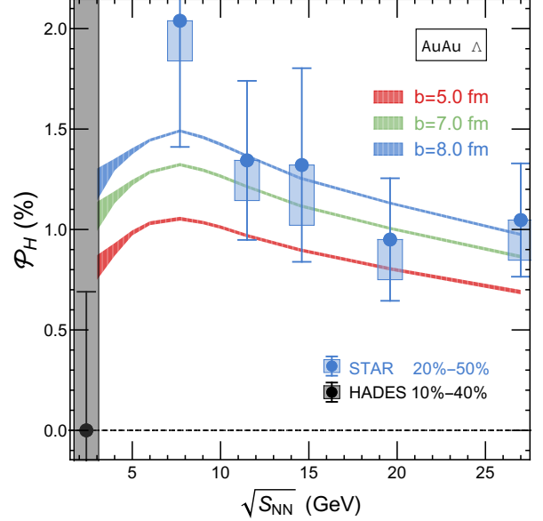
FIG. 1. A global polarization signal as a function of collision beam energy with |y_\Lambda| < 1.0 and 0.4 \text{ GeV} < p_T < 3.0 \text{ GeV} , for AuAu collisions at three different impact parameters b = 5 fm (red), 7 fm (green) and 8 fm (blue), with the bands representing statistical uncertainty from our simulation. Relevant experimental measurements are also shown, with the STAR data from Ref.[1] and the HADES data from Ref. [59].
