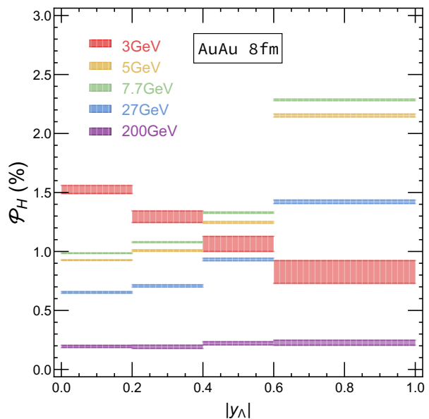
FIG. 3. A global polarization signal as a function of rapidity with 0.4\text{ GeV} < p_T < 3.0\text{ GeV} , for AuAu collisions at impact parameter b = 8\text{ fm} for a variety of collision beam energy from 200 GeV down to 3 GeV, with the bands representing statistical uncertainty from our simulation.
