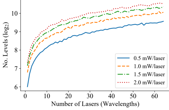
Figure 3. Noise analysis of for photonic dot products independent of crosstalk. Noise has a much lower influence on precision than crosstalk.
