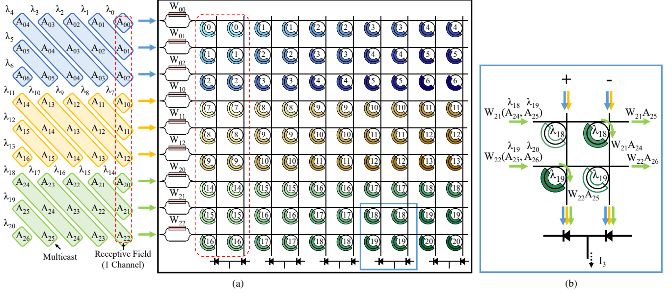
Figure 5. (a) The proposed PLCU with N_m = 9 and N_d = 5 . The overlapping receptive fields produce a multicast pattern. (b) Select signals being switched by MRRs and accumulated at the balanced PDs.
