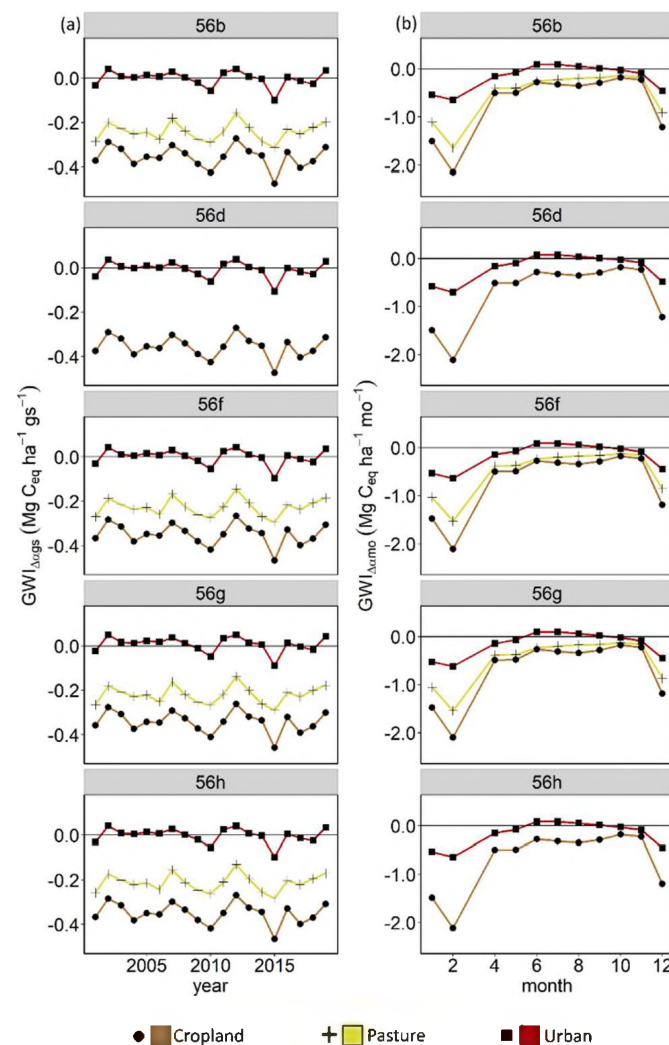
Figure 4. Albedo-induced global warming impact ( \text{GWI}_{\Delta\alpha} ) for a given cover type within the five Level IV ecoregions. Panels (a,b) represent the \text{GWI}_{\Delta\alpha} for the growing season ( \text{GWI}_{\Delta\alpha\text{gs}} ; 2001–2019) and monthly ( \text{GWI}_{\Delta\alpha\text{mo}} ; January–December, less March) periods, respectively. Positive and negative values of \text{GWI}_{\Delta\alpha} indicate warming and cooling effects, respectively, equivalent to Carbon ( \text{C}_{\text{eq}} ) emission and mitigation, respectively.
