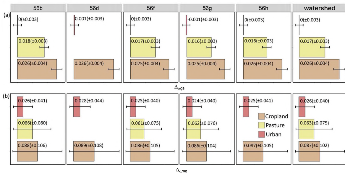
Figure 2. Albedo difference ( \Delta\alpha ) between a cover type i and the forest for (a) growing season ( \Delta\alpha_{gs} ) and (b) monthly ( \Delta\alpha_{mo} ) periods, within the five Level IV ecoregions and the entire Kalamazoo River Watershed 2001–2019. Annotations indicate mean ( \pm standard deviation) of \Delta\alpha_{gs} and \Delta\alpha_{mo} .
