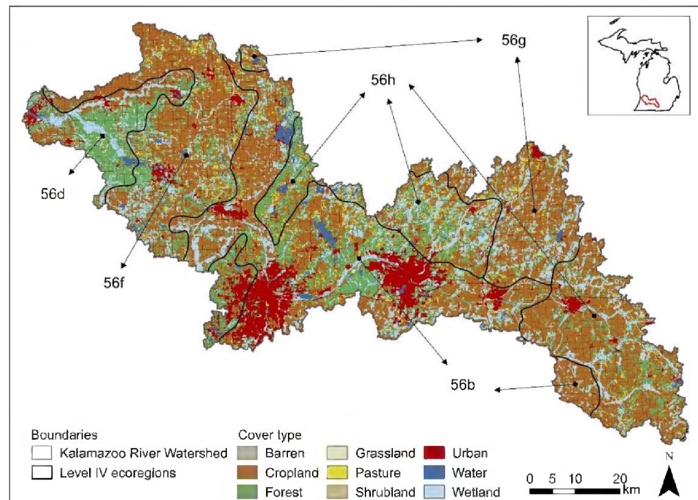
Figure 1. The study area of the five United States Environmental Protection Agency Level IV ecoregions and the nine National Land Cover Database cover type classes within the Kalamazoo River Watershed in 2001. (Map projection: WGS-84 UTM Zone 16 N).
