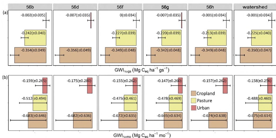
Figure 3. Albedo-induced global warming impact ( GWI_{\Delta\alpha} ) for (a) growing season ( GWI_{\Delta\alpha_{gs}} ) and (b) monthly ( GWI_{\Delta\alpha_{mo}} ) periods, within the five Level IV ecoregions and the entire Kalamazoo River Watershed 2001–2019. Annotations indicate mean ( \pm standard deviation) of GWI_{\Delta\alpha_{gs}} and GWI_{\Delta\alpha_{mo}} .
