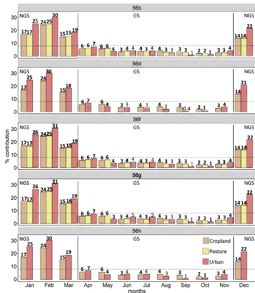
Figure 6. Percent contribution of albedo-induced global warming impact ( GWI_{\Delta\alpha} ) to cooling (values in bold) or warming effects by season and month periods for major cover types in the five Level IV ecoregions. The horizontal dashed line represents the average contribution ~8% (i.e., 1/12 of the annual total), and the solid vertical lines separate the non-growing season (NGS) from the growing season (GS) months. Values of March were missing and gap-filled as the mean GWI_{\Delta\alpha} of February and April.
