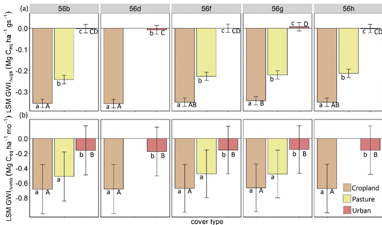
Figure 5. The least square means (LSMs) multi-comparison analysis of albedo-induced global warming impact ( \text{GWI}_{\Delta\alpha} ) for a given cover type across the five Level IV ecoregions for the (a) growing season ( \text{GWI}_{\Delta\alpha\text{gs}} ; 2001–2019) and (b) monthly ( \text{GWI}_{\Delta\alpha\text{mo}} ; January–December) periods. Whiskers represent the lower and upper limits of the 95% family-wise confidence level of the LSMs. Bars sharing the same letters are not significantly different according to the post-hoc Tukey test analysis. Lowercase letters indicate differences among cover types within the five ecoregions, while uppercase letters indicate differences of same cover type among the five ecoregions. The among ecoregions analysis only considered cropland and urban covers (i.e., the cover types that were in every ecoregion).
