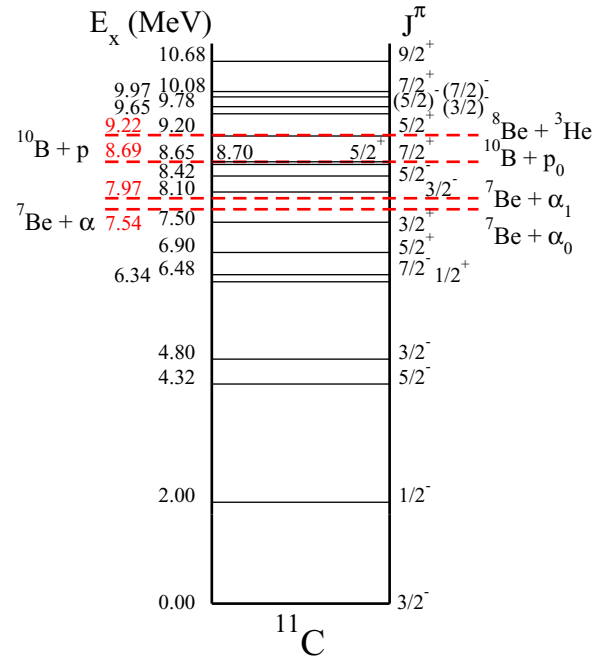
FIG. 1. Level diagram of the ^{11}\text{C} system up to E_x \approx 11 MeV as given in the Evaluated Nuclear Structure Data File (ENSDF) evaluation [42]. The red dashed lines indicate particle separation energies.
