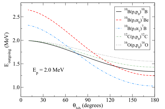
FIG. 2. Energies of outgoing particles for ^{10}\text{B} + p and ^{12}\text{C}(p, p) and ^{16}\text{O}(p, p) reactions at E_p = 2.0 MeV. The similar outgoing particle energies over the central angular range complicates measurements from E_p = 0.8 to 3.0 MeV.
