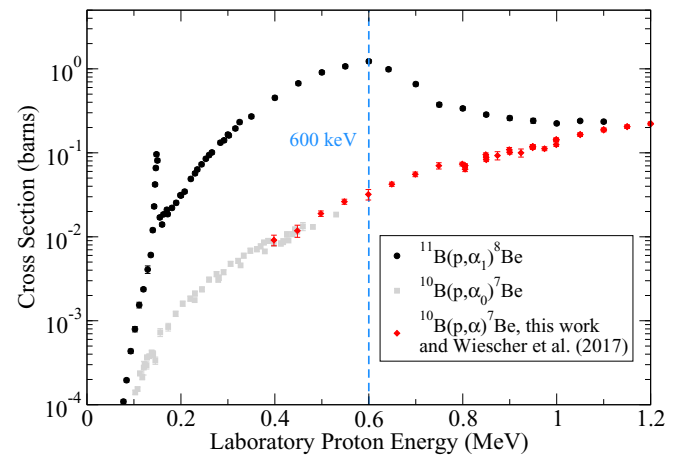
FIG. 15. Comparison of the ^{11}\text{B}(p, \alpha)^8\text{Be} [14] (black circles) and ^{10}\text{B}(p, \alpha_0)^7\text{Be} [21,28,30] (grey squares) cross section data over the energy range of interest for aneutronic fusion applications. The present ^{10}\text{B}(p, \alpha)^7\text{Be} total cross section data are indicated by the red diamonds.
