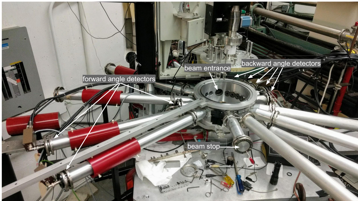
FIG. 5. Ohio University experimental setup. Particle detectors were placed at the end of the extension pipes that have been installed off of the main section of the scattering chamber. The larger distance between detector and target is required in order to provide sufficient resolution for particle identification using ToF. See text for details.
