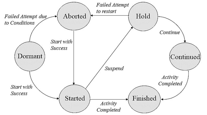
Figure 3: States of an Activity
