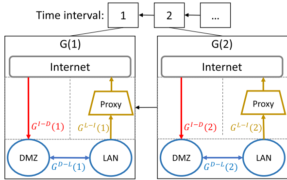
Fig. 4. Data structure for T-CSM.
