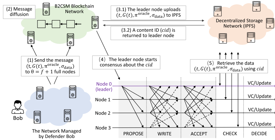
Fig. B.3. The message flow of the cyber data replication phase in B2CSM system.
