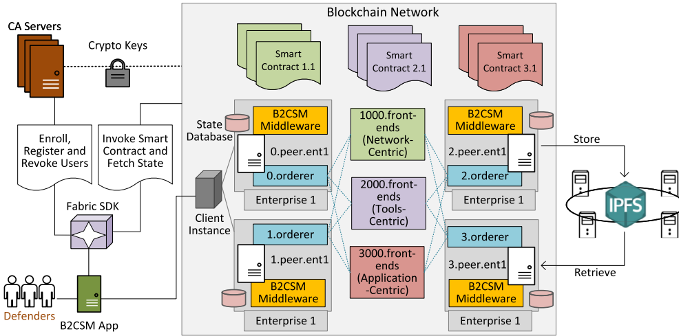
Fig. 11. Illustration of the B2CSM prototype system with 4 blockchain peer nodes, on which a private channel is created for one enterprise. Each node also acts as a replica of the BFT SMaRt-based ordering service and has a couchdb database. For method \mathcal{M}_2 , the B2CSM middleware also contacts with IPFS for cyber data writing and retrieval. The cases for 7 or 10 ordering (or peer) nodes follow the similar architecture and multiple-enterprise architecture can also be easily switched.
