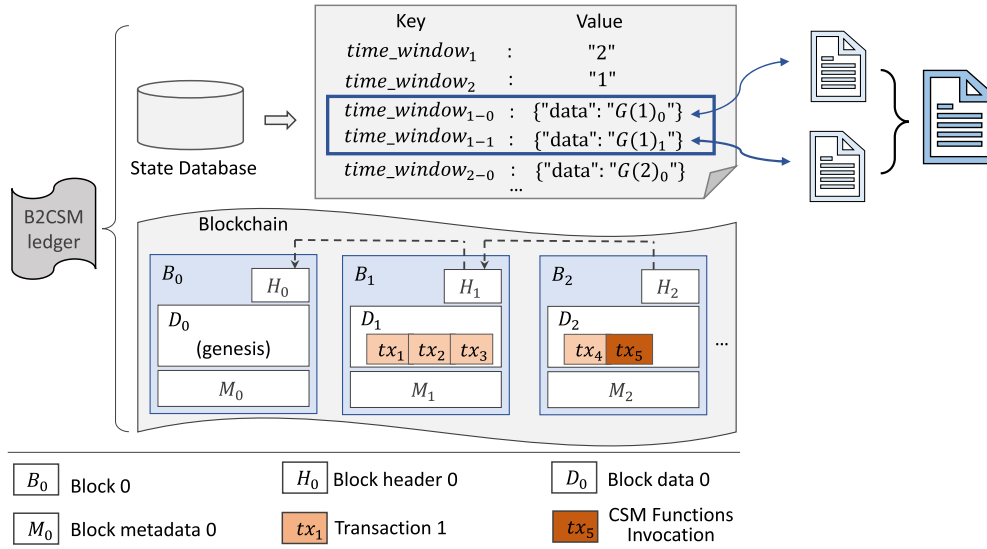
Fig. 9. Illustration of the B2CSM ledger structure with a blockchain and a state database. The state database stores the cyber data units.
