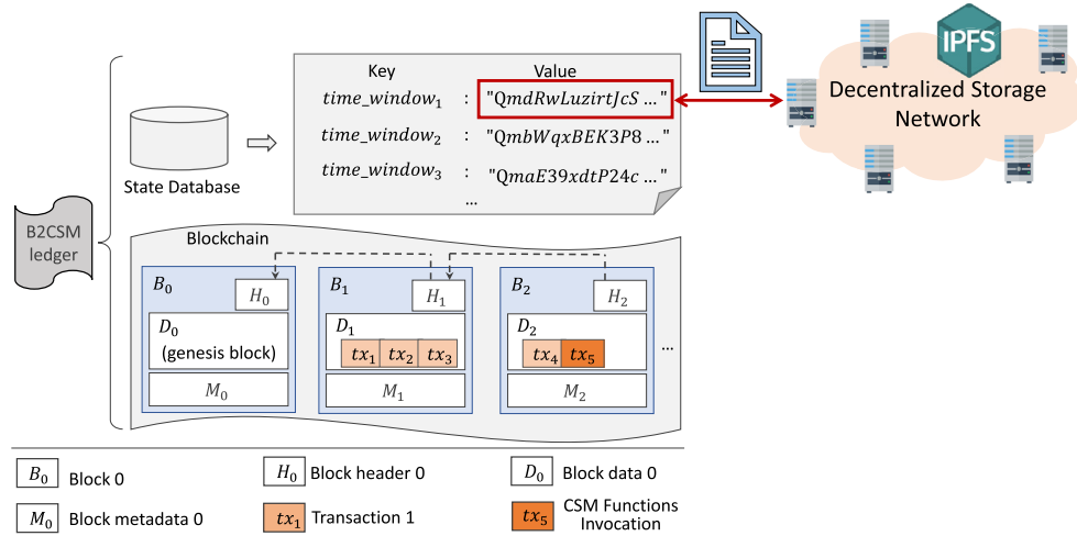
Fig. 10. Illustration of the B2CSM ledger structure with a blockchain and a state database. The state database stores content id cid of the cyber data that is returned by IPFS.
