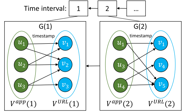
Fig. 5. Data structure for A-CSM.
