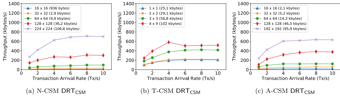
Fig. 12. B2CSM's DRT CSM in different CSM experiments (averaged over 5 independent runs).
