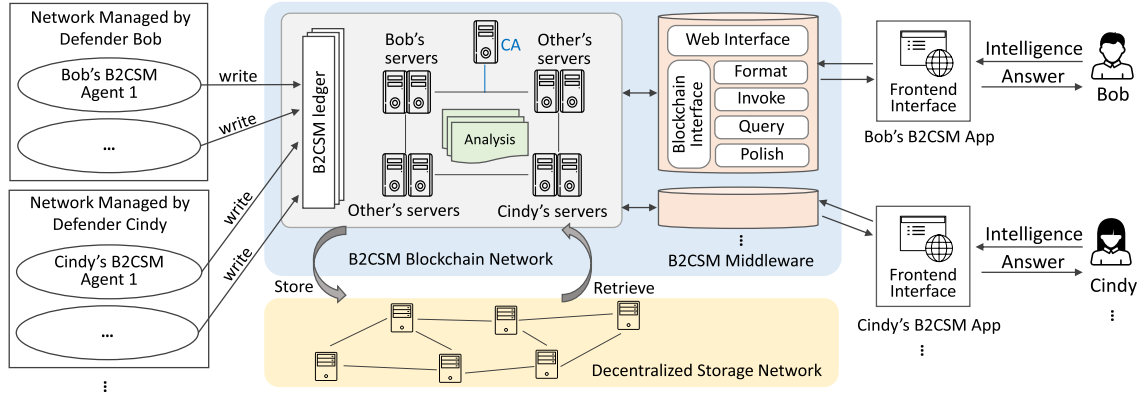
Fig. B.2. Illustration of B2CSM architecture based on Blockchain and decentralized storage network.
