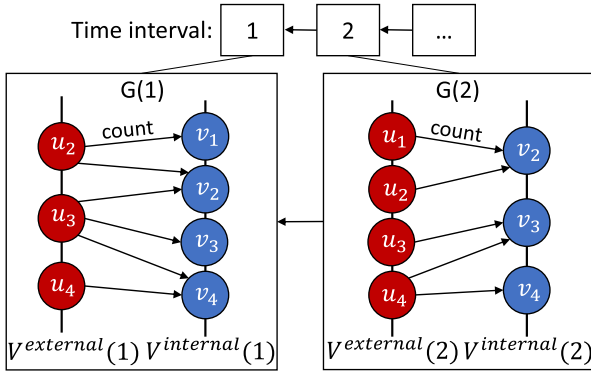
Fig. 3. Data structure for N-CSM.
