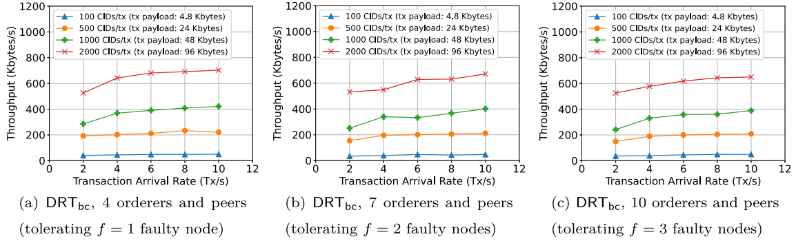
Fig. 14. B2CSM's DRT bc with different number of orderers (averaged over 5 independent runs).
