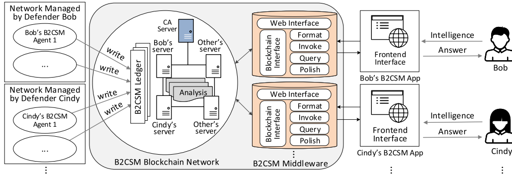
Fig. 7. Illustration of B2CSM architecture. Each defender has a set of agents for collecting cyber data and writing into the B2CSM blockchain (either via the B2CSM Middleware or an independent writing module). Each defender runs a B2CSM App, which invokes CSM functions deployed in the smart contract using cyber intelligence from the defender.
