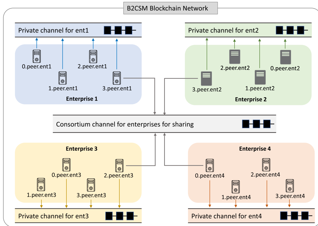
Fig. 8. The channel architecture in B2CSM blockchain network. The private and consortium channels can further serve different classes of CSM, i.e., N-CSM, T-CSM or A-CSM.
