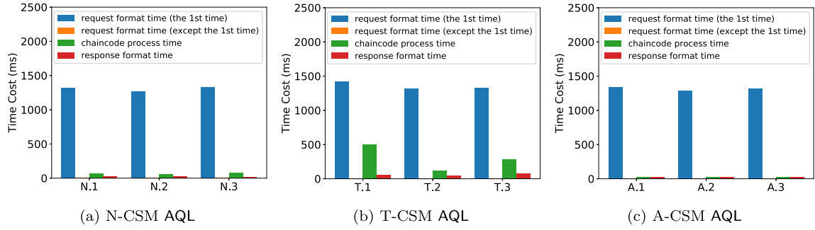
Fig. 13. B2CSM's AQL in different CSM cases (averaged over 5 independent runs).
