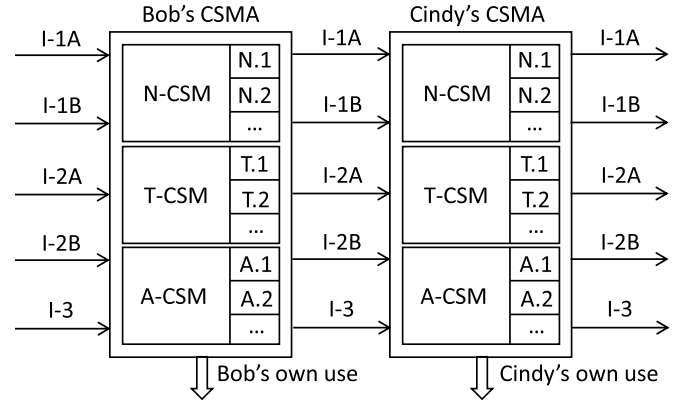
Fig. 2. CSM model with five kinds of input cyber intelligence and three classes of CSM functions. The naming scheme is: '1' means attacker, '2' means victim, and '3' means capabilities; 'A' means intelligence on external entities and 'B' means intelligence on internal entities.
