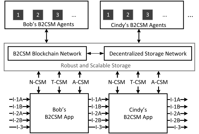
Fig. B.1. The B2CSM model extending from the CSM model using method \mathcal{M}_2 .
