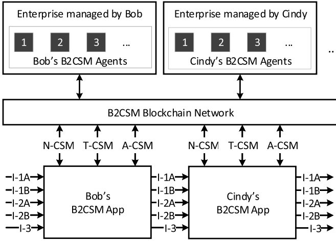
Fig. 6. The B2CSM model extending from the CSM model.
