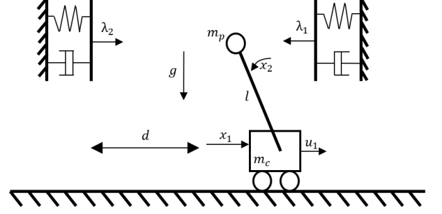
Fig. 2. Benchmark problem: Regulation of the cart-pole system to the origin with soft walls.
