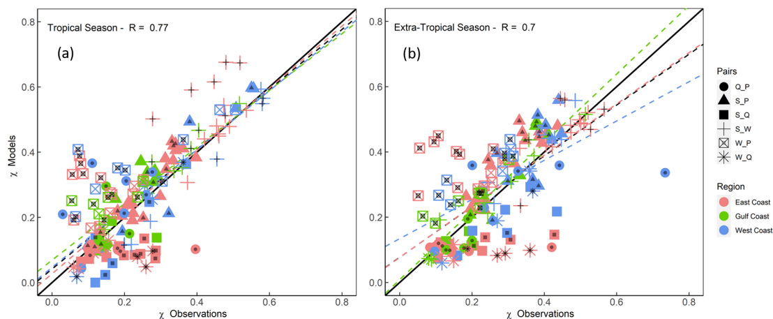
Figure 11. Scatterplot comparing extremal (tail) dependence (for q = 0.9 ) derived using observations (x axis) and models (y axis) for tropical (a) and extra-tropical (b) seasons, using a daily time series of both variables. Colours denote the location (separated into East, Gulf, and West coasts), and markers represent the different variable pairs. Black dots on markers indicate significant difference in the tail dependence structure between observations and models according to the KL divergence. Dashed lines show linear regression fits corresponding to all data points (black) and for different subsets according to locations (coloured as outlined in the legend).
