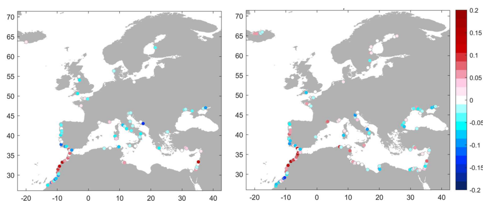
Figure 6: Differences in the Kendall's correlation coefficient ( p < 0.05 ) obtained when using Q and SW and Q and WL (left panel) and P and SW and P and WL (right panel) when SW or WL are the dominant variables.
