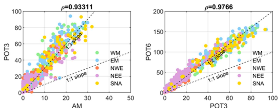
Figure 3: a) Scatter plots of the number of co-occurring events between Q and P using AM vs POT3 (left panel) and using POT3 vs POT6 (right panel). Dashed lines mark relationships between AM and POT3 or between POT3 and POT6 covering scaling factors equal to 2.0 and 3.0.
