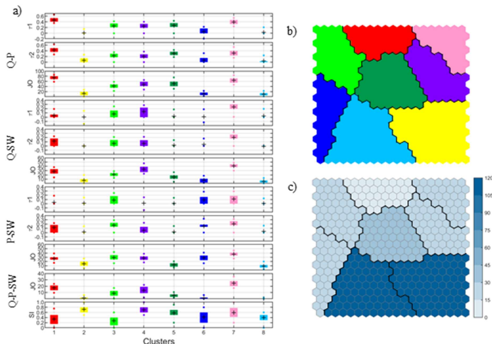
Figure 10: KMA classification: a) Characteristics of each cluster: \tau(Q-P) , \tau(P-Q) , Co(Q-P) , \tau(Q-SW) , \tau(SW-Q) , Co(Q-SW) , \tau(P-SW) , \tau(SW-P) , Co(P-SW) , Co(Q-P-SW) , SI ; b) The 8 KMA clusters over the SOM lattice; c) Number of locations represented by each KMA cluster.
