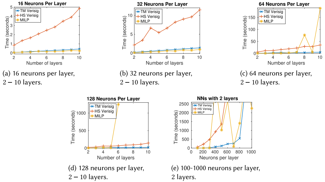
Fig. 9. Comparison in terms of verification times between the two versions of Verisig and the MILP-based approach. In 9(a)–(d), the number of neurons is fixed and number of layers varies from two to 10. In (e), the number of layers is fixed to two, and the number of neurons varies from 100 to 1,000.
