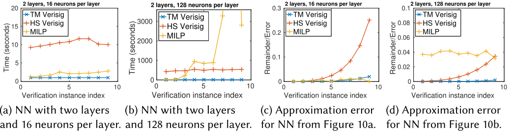
Fig. 10. Comparison in terms of verification times (Figure 10(a) and (b)) and approximation error (Figure 10(c) and (d)) between the two versions of Verisig and the MILP-based approach. In each figure, the initial set uncertainty is gradually increased with the instance index.
