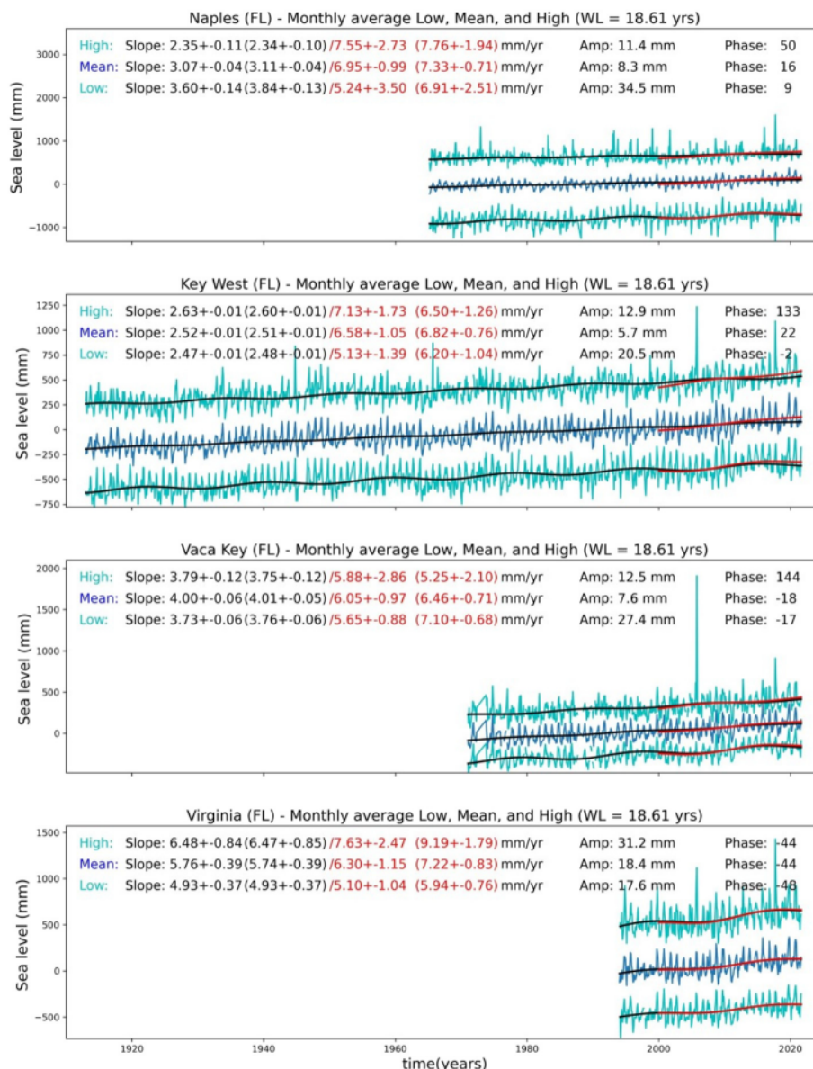
Fig. 2. Historical (all available data) and recent (2000–2021) mean high, mean, and mean low water level records of four South Florida NOAA tide stations. Best-fit parameter estimation of the historical data are shown in black fonts and recent (2000–2021) in red fonts. Values without parenthesis present the linear + periodic fit and those within the parenthesis present trends of the linear fit. (For interpretation of the references to colour in this figure legend, the reader is referred to the web version of this article.)
