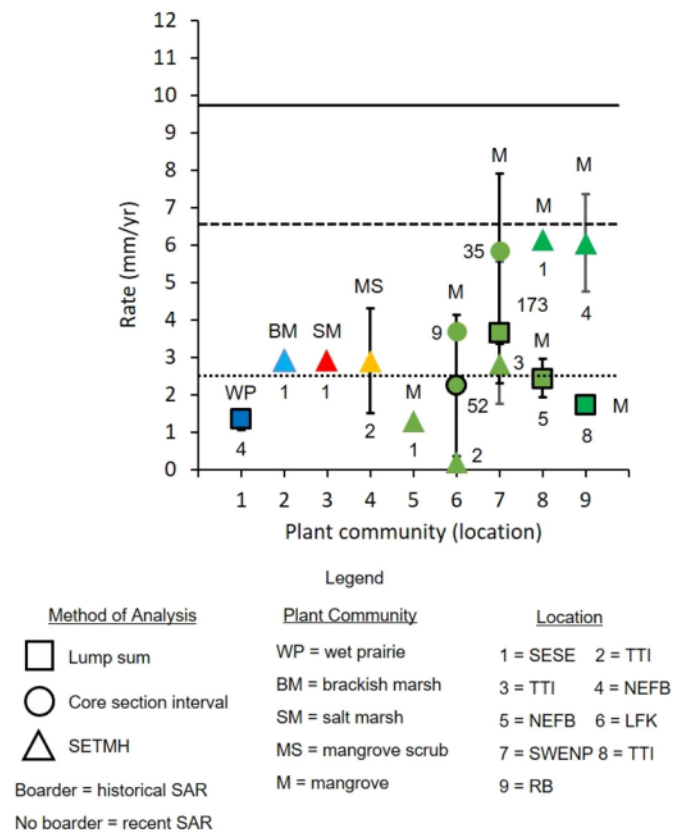
Fig. 4. Mean sediment accumulation rates plotted as a function of (1) coastal wetland plant community type, (2) method of analysis (e.g., lump sum and core section interval radioisotope geochronologies [Pb210, Cs137], Sediment Elevation Table Marker Horizon [SETMH]), and (3) timeframe (historical, 1900–2021; recent, 2000–2021; and past decade, 2010–2021). Horizontal dotted line = Key West historical (1913–2021) rate of SLR (2.5 mm yr -1 ). Horizontal dashed line = Key West recent (2000–2021) rate of SLR (6.6 mm yr -1 ). Horizontal solid line = Key West past decade (2010–2021) rate of SLR (9.7 mm yr -1 ). Error bars = 1 S.D. N value associated with each series is number of sediment samples used to calculate mean sediment accumulation rate.
